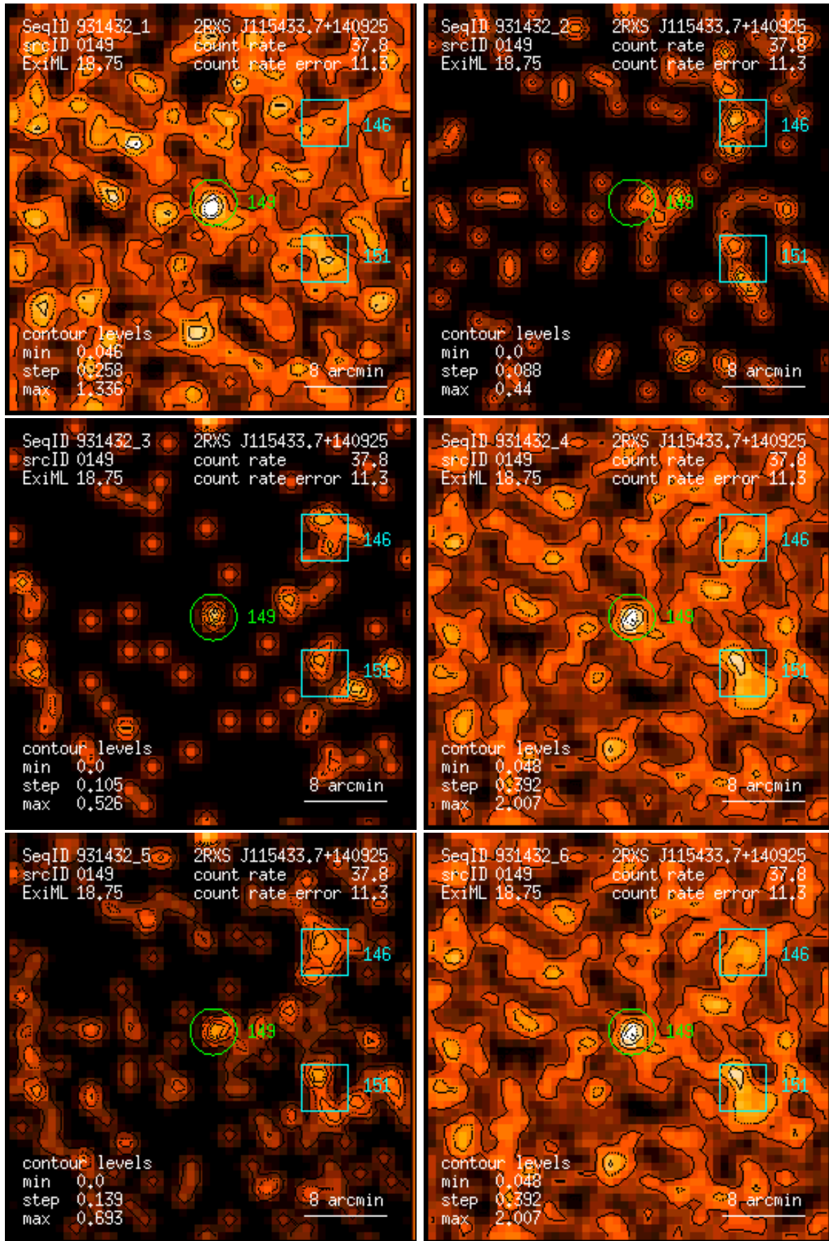
Figure 149: RASS 931432: detection 0149: band rate images, Gaussian filter: (1) PSPC channels 11 – 41, (2) 52 – 90, (3) 91 – 201, (4) 11 – 235, (5) 52 – 201, (6) 11 – 201. Broad band rates in counts/ks. Band rate contour levels in counts/ks/arcmin 2 .
