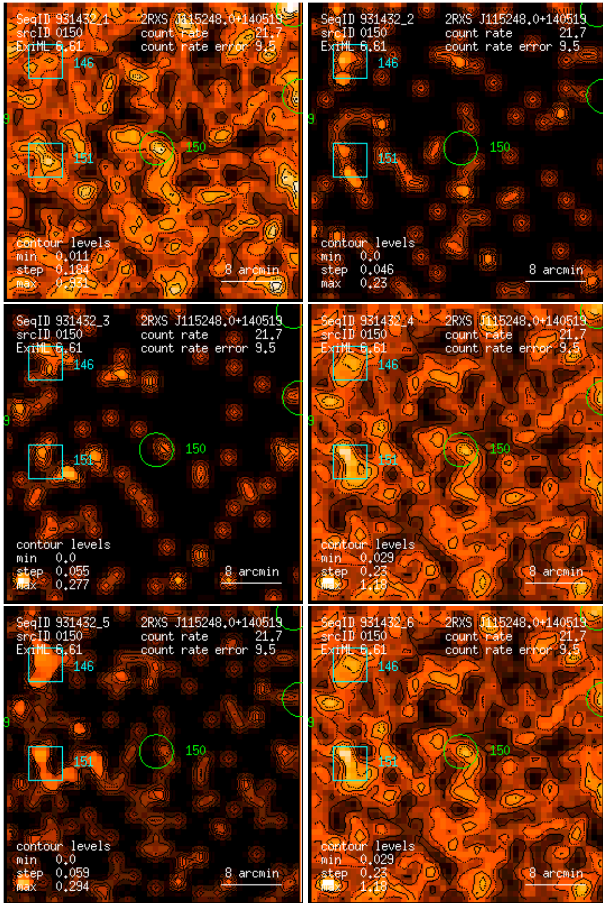
Figure 150: RASS 931432: detection 0150: band rate images, Gaussian filter: (1) PSPC channels 11 – 41, (2) 52 – 90, (3) 91 – 201, (4) 11 – 235, (5) 52 – 201, (6) 11 – 201. Broad band rates in counts/ks. Band rate contour levels in counts/ks/arcmin 2 .
