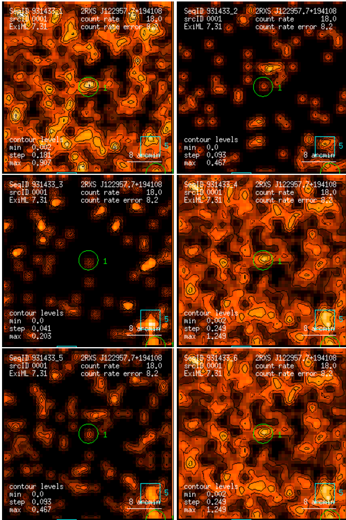
Figure 1: RASS 931433: detection 0001: band rate images, Gaussian filter: (1) PSPC channels 11 – 41, (2) 52 – 90, (3) 91 – 201, (4) 11 – 235, (5) 52 – 201, (6) 11 – 201. Broad band rates in counts/ks. Band rate contour levels in counts/ks/arcmin 2 .
