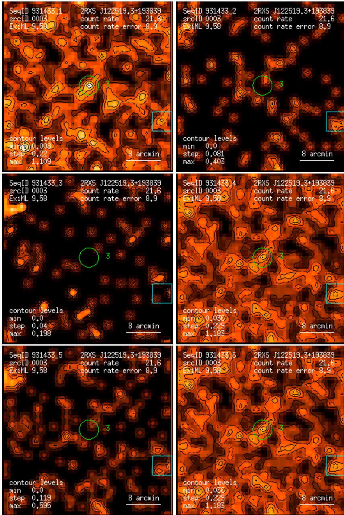
Figure 3: RASS 931433: detection 0003: band rate images, Gaussian filter: (1) PSPC channels 11 – 41, (2) 52 – 90, (3) 91 – 201, (4) 11 – 235, (5) 52 – 201, (6) 11 – 201. Broad band rates in counts/ks. Band rate contour levels in counts/ks/arcmin 2 .
