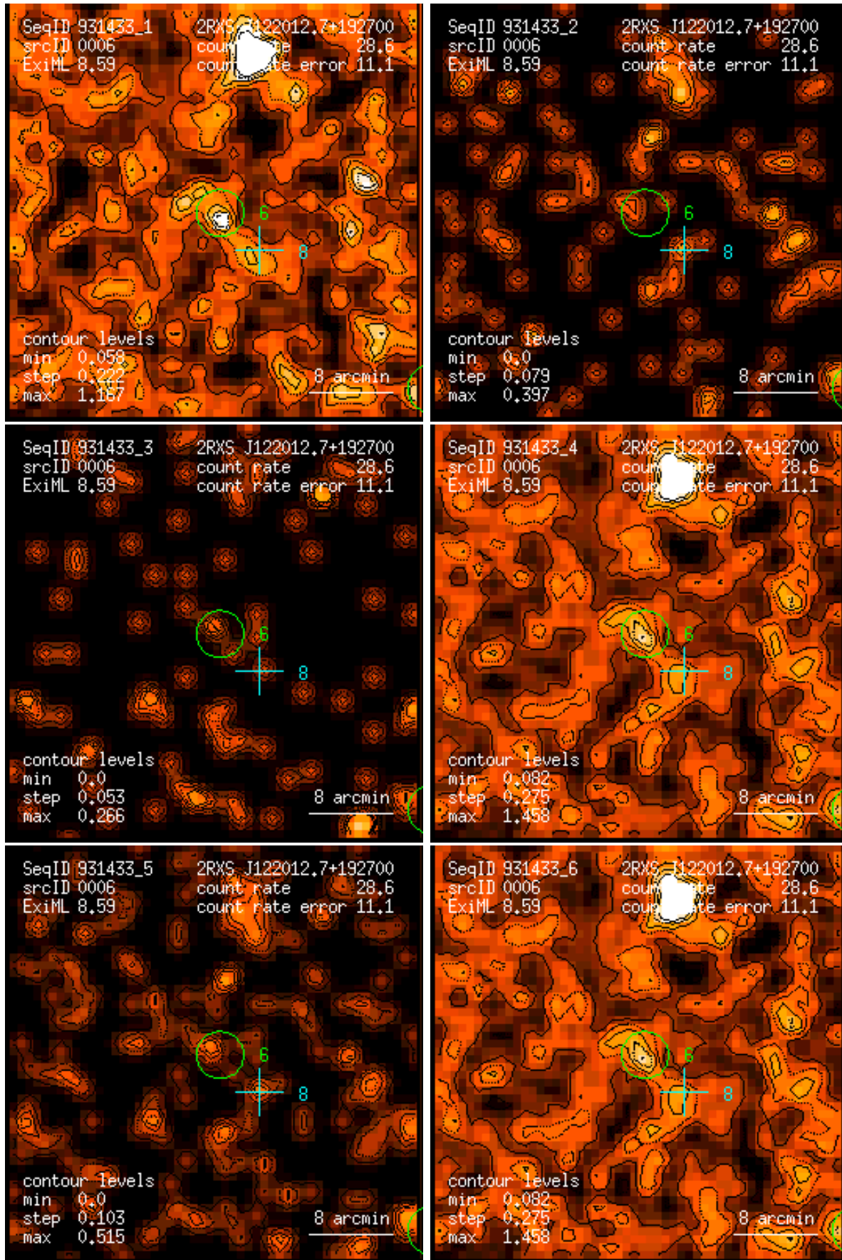
Figure 6: RASS 931433: detection 0006: band rate images, Gaussian filter: (1) PSPC channels 11 – 41, (2) 52 – 90, (3) 91 – 201, (4) 11 – 235, (5) 52 – 201, (6) 11 – 201. Broad band rates in counts/ks. Band rate contour levels in counts/ks/arcmin 2 .
