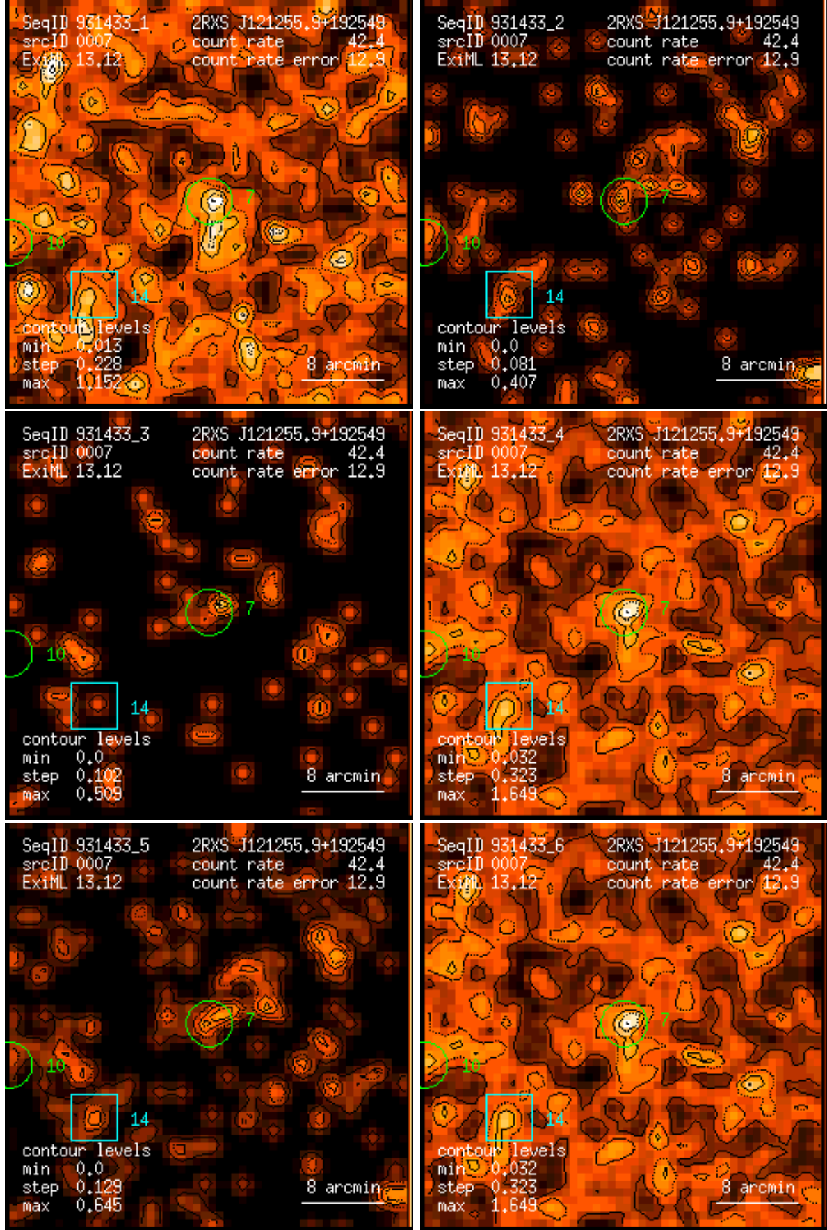
Figure 7: RASS 931433: detection 0007: band rate images, Gaussian filter: (1) PSPC channels 11 – 41, (2) 52 – 90, (3) 91 – 201, (4) 11 – 235, (5) 52 – 201, (6) 11 – 201. Broad band rates in counts/ks. Band rate contour levels in counts/ks/arcmin 2 .
