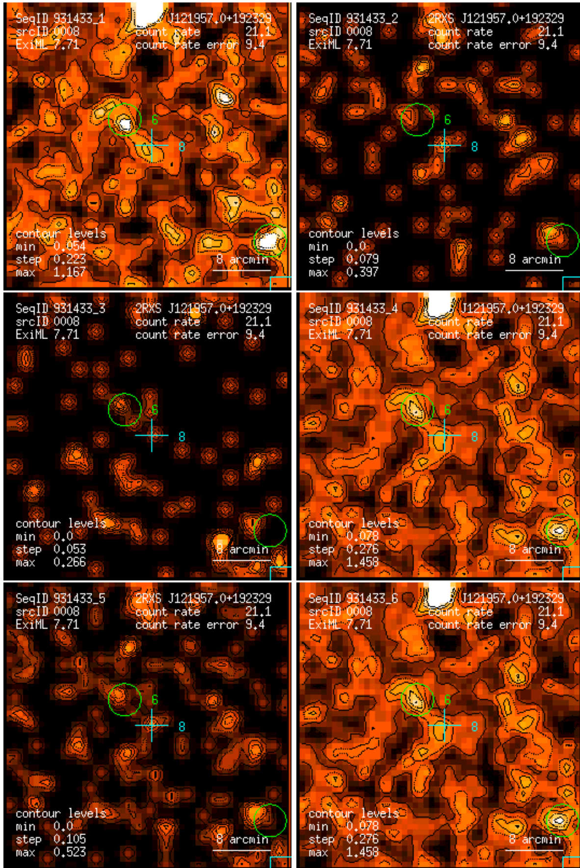
Figure 8: RASS 931433: detection 0008: band rate images, Gaussian filter: (1) PSPC channels 11 – 41, (2) 52 – 90, (3) 91 – 201, (4) 11 – 235, (5) 52 – 201, (6) 11 – 201. Broad band rates in counts/ks. Band rate contour levels in counts/ks/arcmin 2 .
