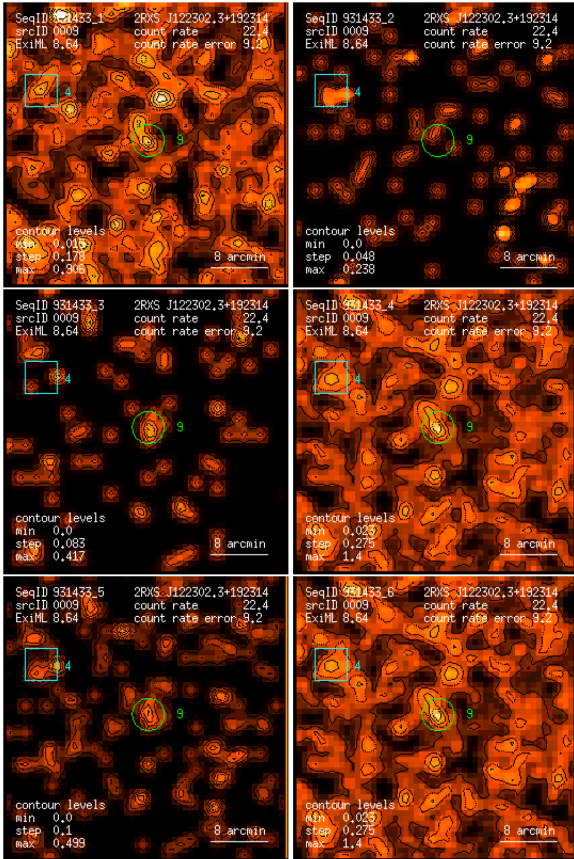
Figure 9: RASS 931433: detection 0009: band rate images, Gaussian filter: (1) PSPC channels 11 – 41, (2) 52 – 90, (3) 91 – 201, (4) 11 – 235, (5) 52 – 201, (6) 11 – 201. Broad band rates in counts/ks. Band rate contour levels in counts/ks/arcmin 2 .
