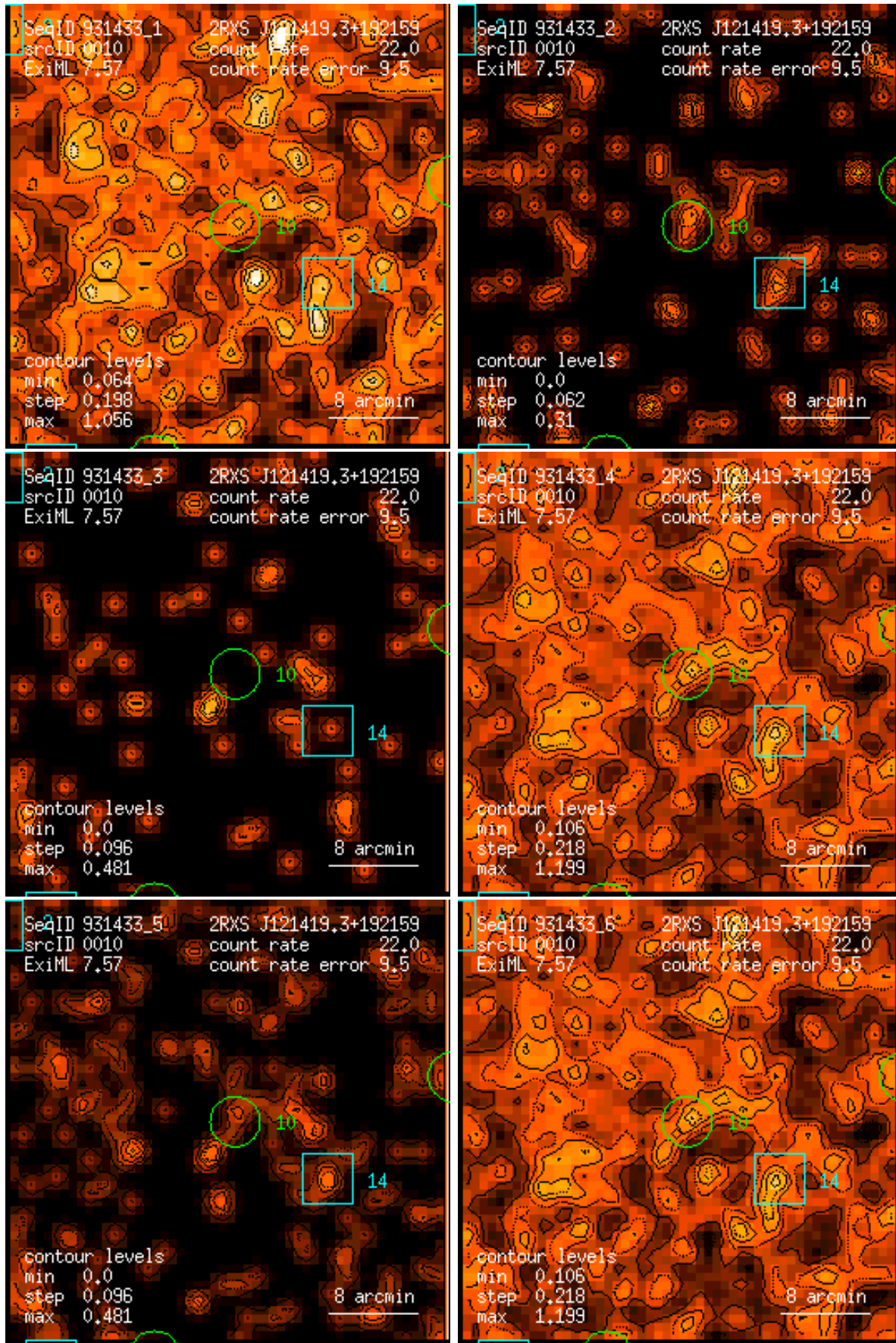
Figure 10: RASS 931433: detection 0010: band rate images, Gaussian filter: (1) PSPC channels 11 – 41, (2) 52 – 90, (3) 91 – 201, (4) 11 – 235, (5) 52 – 201, (6) 11 – 201. Broad band rates in counts/ks. Band rate contour levels in counts/ks/arcmin 2 .
