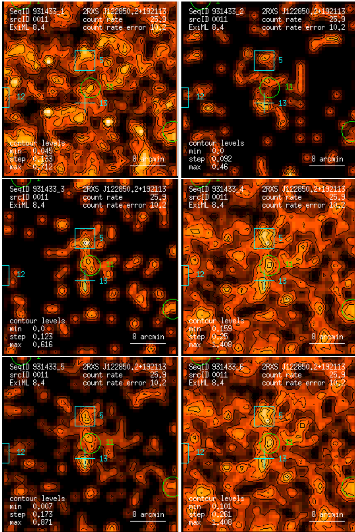
Figure 11: RASS 931433: detection 0011: band rate images, Gaussian filter: (1) PSPC channels 11 – 41, (2) 52 – 90, (3) 91 – 201, (4) 11 – 235, (5) 52 – 201, (6) 11 – 201. Broad band rates in counts/ks. Band rate contour levels in counts/ks/arcmin 2 .
