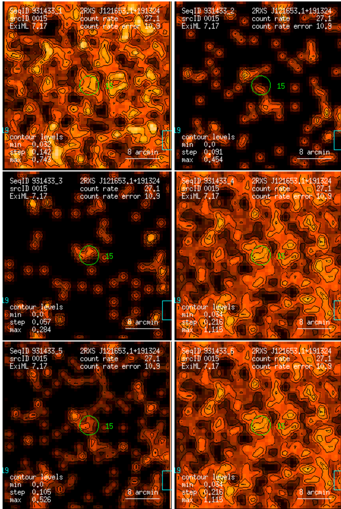
Figure 15: RASS 931433: detection 0015: band rate images, Gaussian filter: (1) PSPC channels 11 – 41, (2) 52 – 90, (3) 91 – 201, (4) 11 – 235, (5) 52 – 201, (6) 11 – 201. Broad band rates in counts/ks. Band rate contour levels in counts/ks/arcmin 2 .
