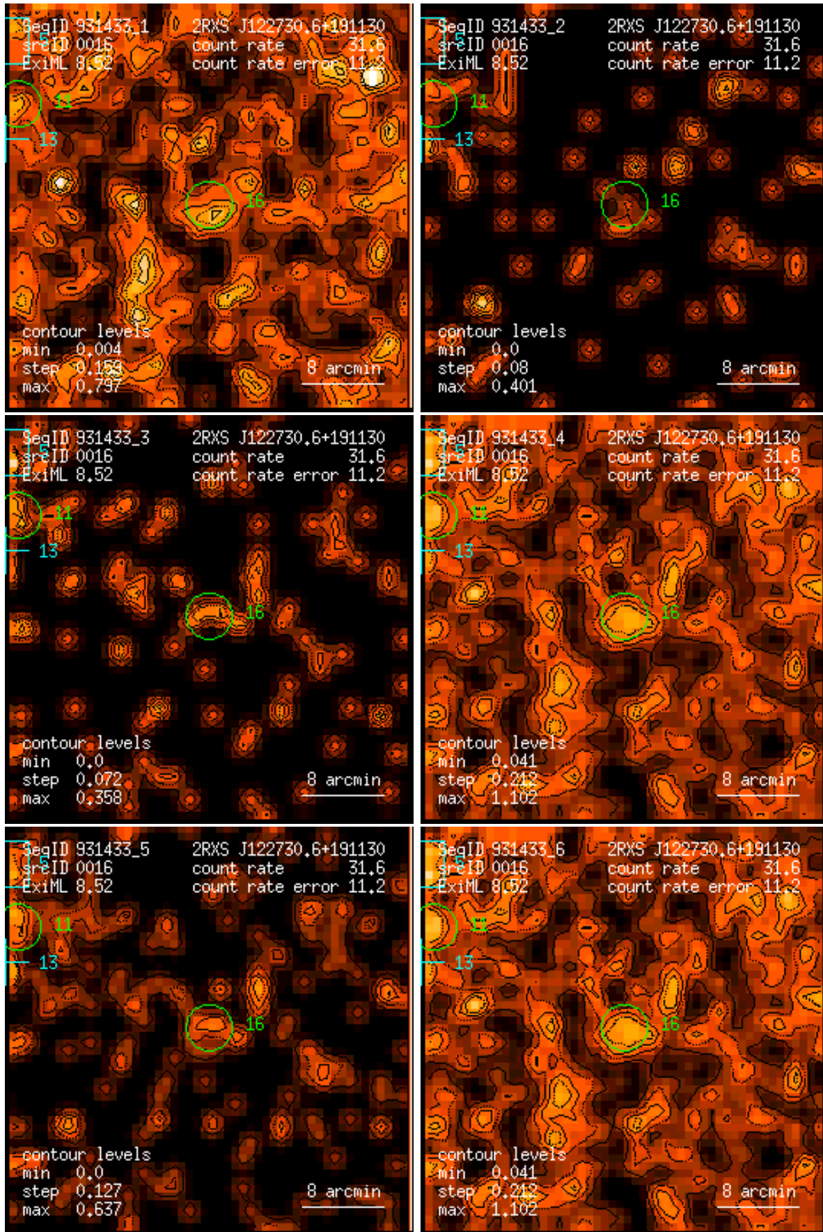
Figure 16: RASS 931433: detection 0016: band rate images, Gaussian filter: (1) PSPC channels 11 – 41, (2) 52 – 90, (3) 91 – 201, (4) 11 – 235, (5) 52 – 201, (6) 11 – 201. Broad band rates in counts/ks. Band rate contour levels in counts/ks/arcmin 2 .
