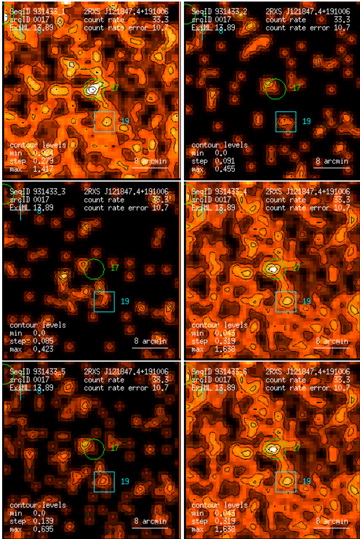
Figure 17: RASS 931433: detection 0017: band rate images, Gaussian filter: (1) PSPC channels 11 – 41, (2) 52 – 90, (3) 91 – 201, (4) 11 – 235, (5) 52 – 201, (6) 11 – 201. Broad band rates in counts/ks. Band rate contour levels in counts/ks/arcmin 2 .
