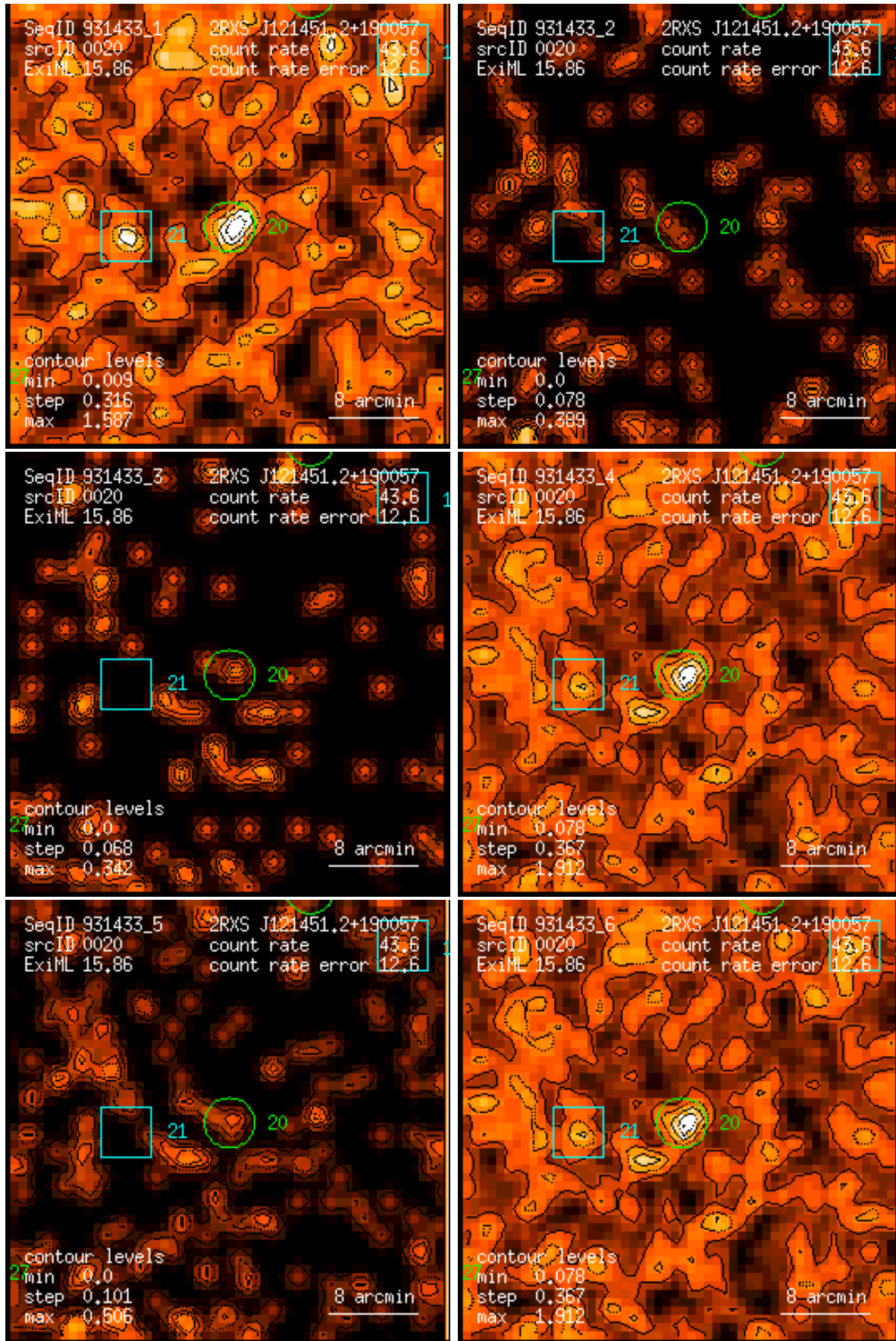
Figure 20: RASS 931433: detection 0020: band rate images, Gaussian filter: (1) PSPC channels 11 – 41, (2) 52 – 90, (3) 91 – 201, (4) 11 – 235, (5) 52 – 201, (6) 11 – 201. Broad band rates in counts/ks. Band rate contour levels in counts/ks/arcmin 2 .
