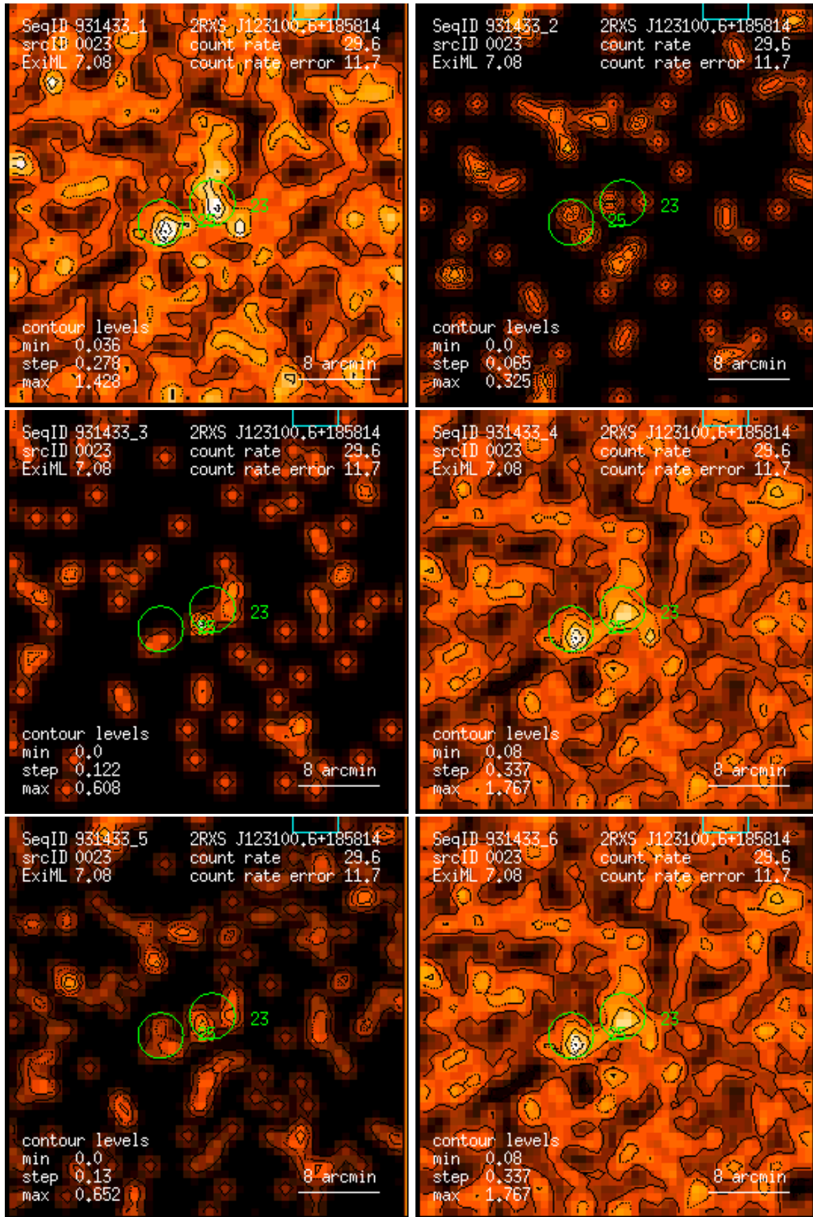
Figure 23: RASS 931433: detection 0023: band rate images, Gaussian filter: (1) PSPC channels 11 – 41, (2) 52 – 90, (3) 91 – 201, (4) 11 – 235, (5) 52 – 201, (6) 11 – 201. Broad band rates in counts/ks. Band rate contour levels in counts/ks/arcmin 2 .
