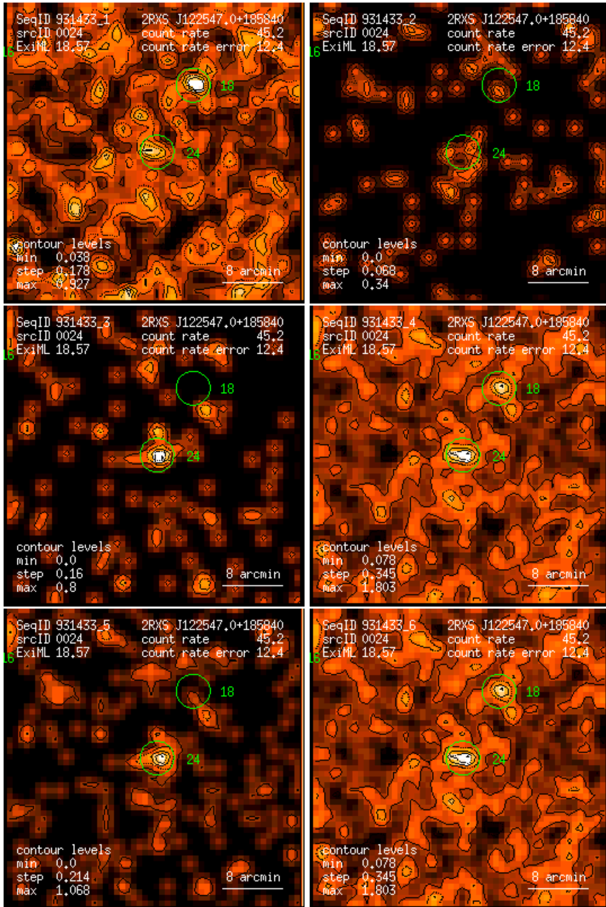
Figure 24: RASS 931433: detection 0024: band rate images, Gaussian filter: (1) PSPC channels 11 – 41, (2) 52 – 90, (3) 91 – 201, (4) 11 – 235, (5) 52 – 201, (6) 11 – 201. Broad band rates in counts/ks. Band rate contour levels in counts/ks/arcmin 2 .
