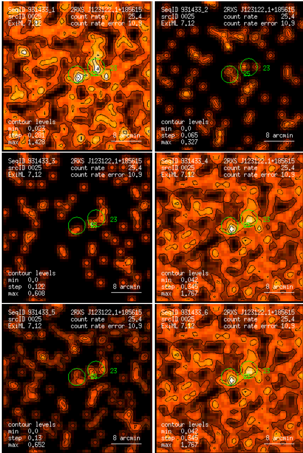
Figure 25: RASS 931433: detection 0025: band rate images, Gaussian filter: (1) PSPC channels 11 – 41, (2) 52 – 90, (3) 91 – 201, (4) 11 – 235, (5) 52 – 201, (6) 11 – 201. Broad band rates in counts/ks. Band rate contour levels in counts/ks/arcmin 2 .
