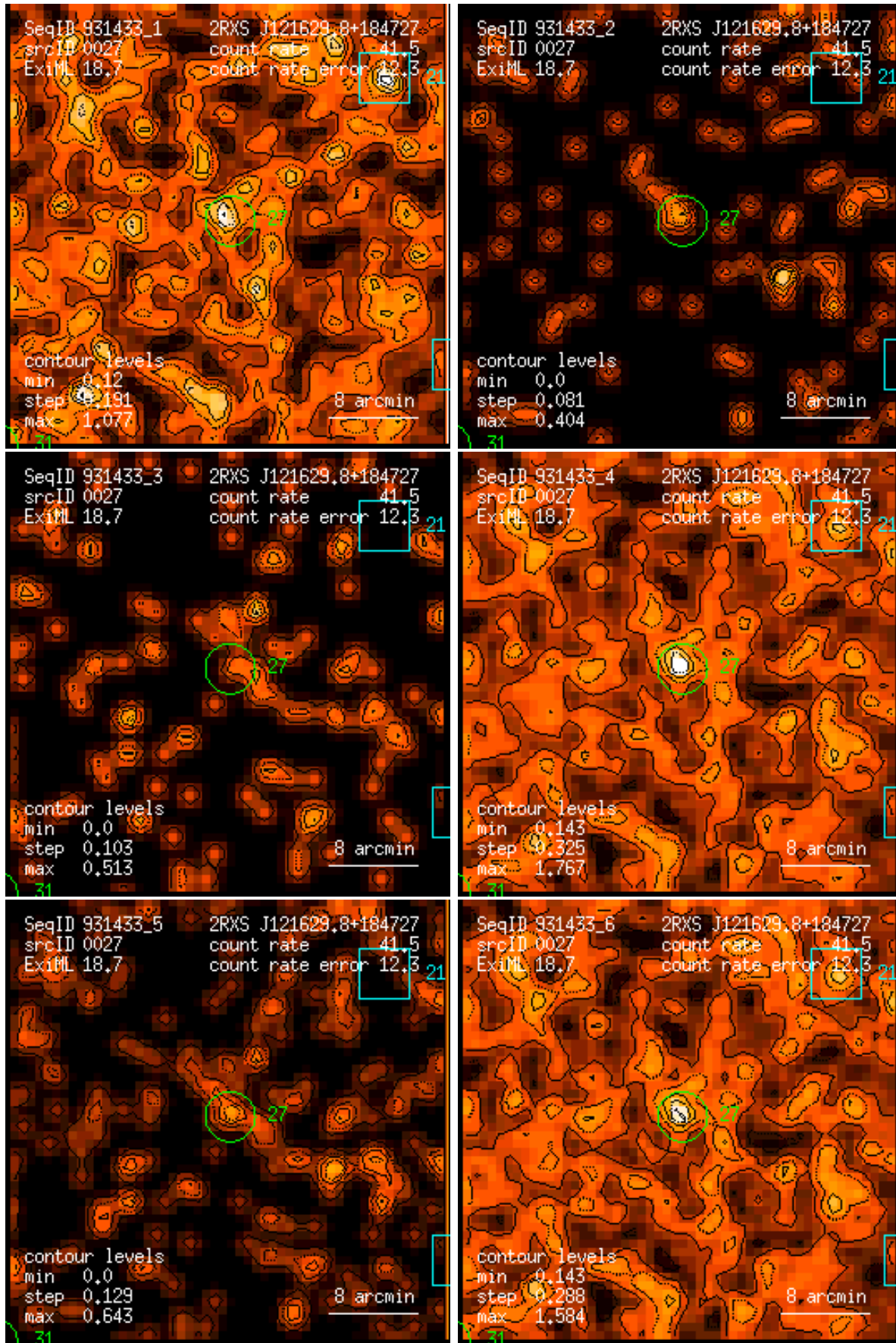
Figure 27: RASS 931433: detection 0027: band rate images, Gaussian filter: (1) PSPC channels 11 – 41, (2) 52 – 90, (3) 91 – 201, (4) 11 – 235, (5) 52 – 201, (6) 11 – 201. Broad band rates in counts/ks. Band rate contour levels in counts/ks/arcmin 2 .
