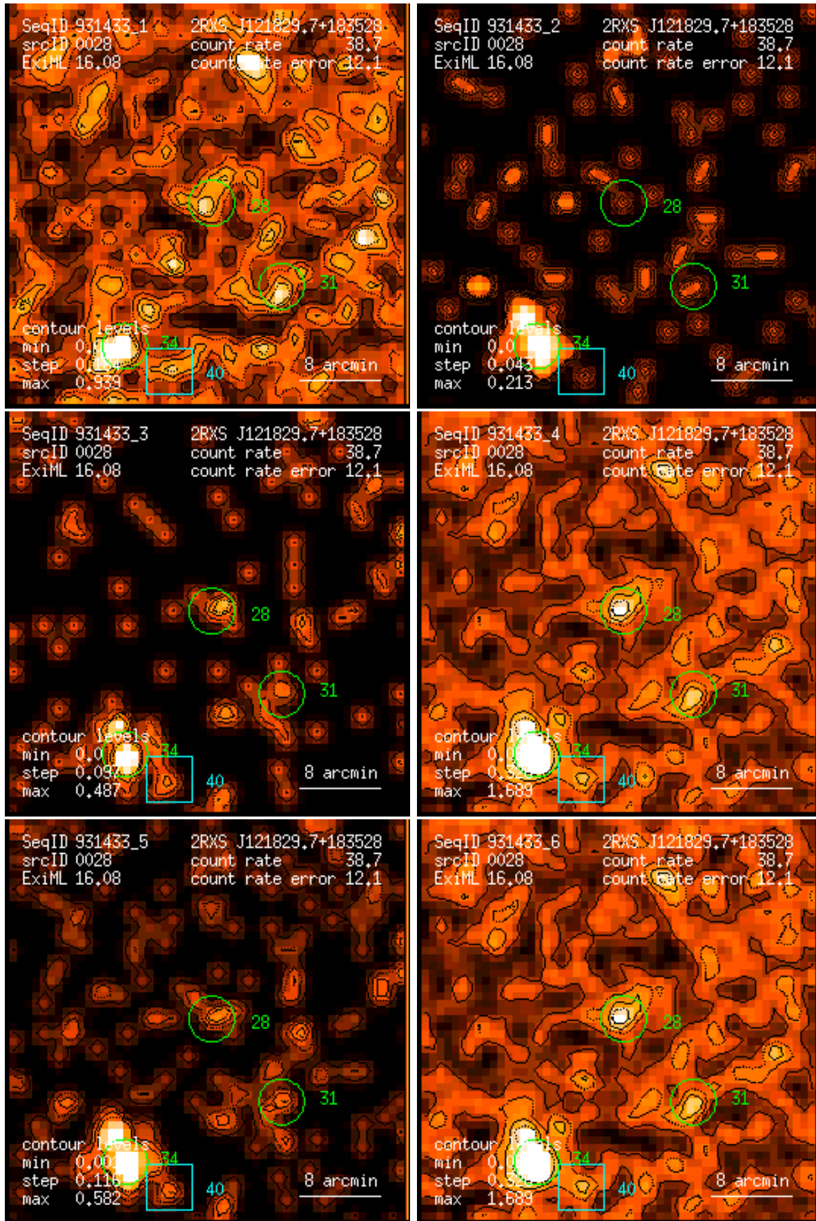
Figure 28: RASS 931433: detection 0028: band rate images, Gaussian filter: (1) PSPC channels 11 – 41, (2) 52 – 90, (3) 91 – 201, (4) 11 – 235, (5) 52 – 201, (6) 11 – 201. Broad band rates in counts/ks. Band rate contour levels in counts/ks/arcmin 2 .
