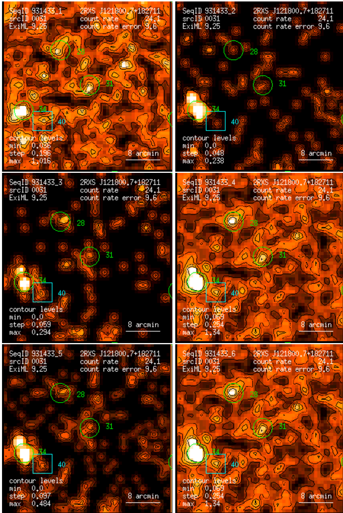
Figure 31: RASS 931433: detection 0031: band rate images, Gaussian filter: (1) PSPC channels 11 – 41, (2) 52 – 90, (3) 91 – 201, (4) 11 – 235, (5) 52 – 201, (6) 11 – 201. Broad band rates in counts/ks. Band rate contour levels in counts/ks/arcmin 2 .
