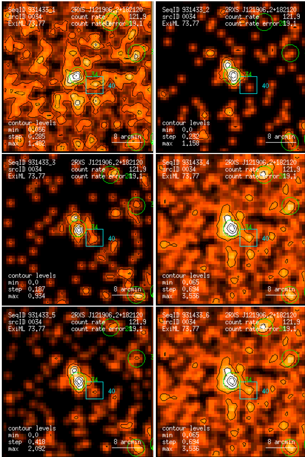
Figure 34: RASS 931433: detection 0034: band rate images, Gaussian filter: (1) PSPC channels 11 – 41, (2) 52 – 90, (3) 91 – 201, (4) 11 – 235, (5) 52 – 201, (6) 11 – 201. Broad band rates in counts/ks. Band rate contour levels in counts/ks/arcmin 2 .
