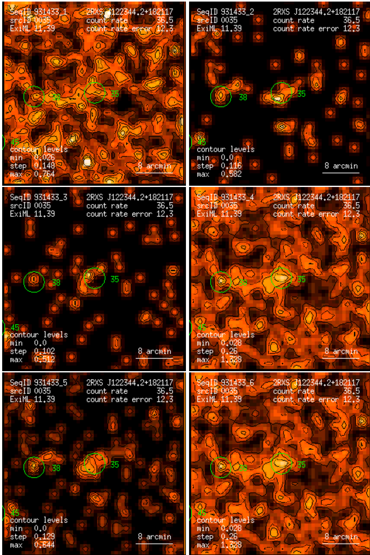
Figure 35: RASS 931433: detection 0035: band rate images, Gaussian filter: (1) PSPC channels 11 – 41, (2) 52 – 90, (3) 91 – 201, (4) 11 – 235, (5) 52 – 201, (6) 11 – 201. Broad band rates in counts/ks. Band rate contour levels in counts/ks/arcmin 2 .
