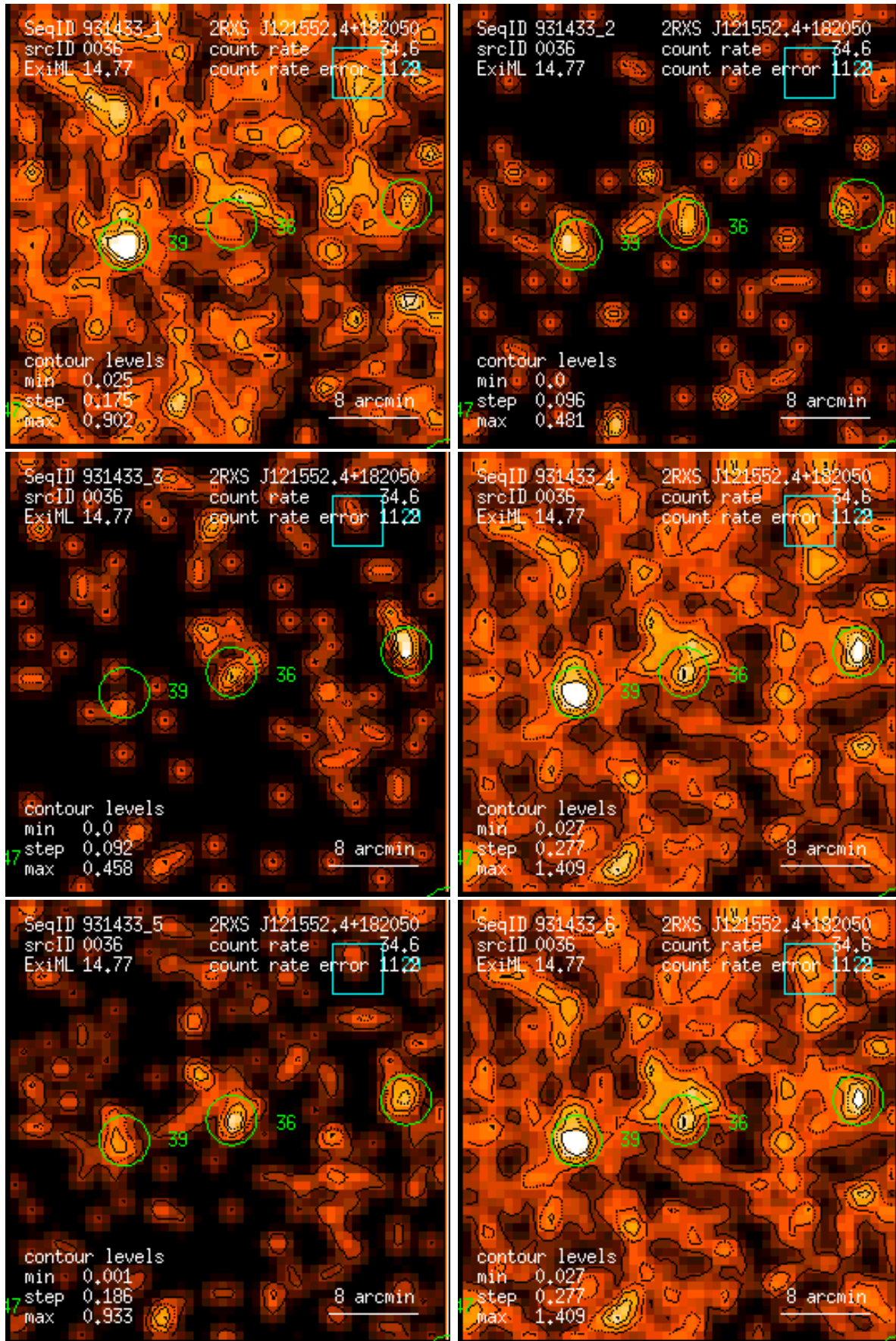
Figure 36: RASS 931433: detection 0036: band rate images, Gaussian filter: (1) PSPC channels 11 – 41, (2) 52 – 90, (3) 91 – 201, (4) 11 – 235, (5) 52 – 201, (6) 11 – 201. Broad band rates in counts/ks. Band rate contour levels in counts/ks/arcmin 2 .
