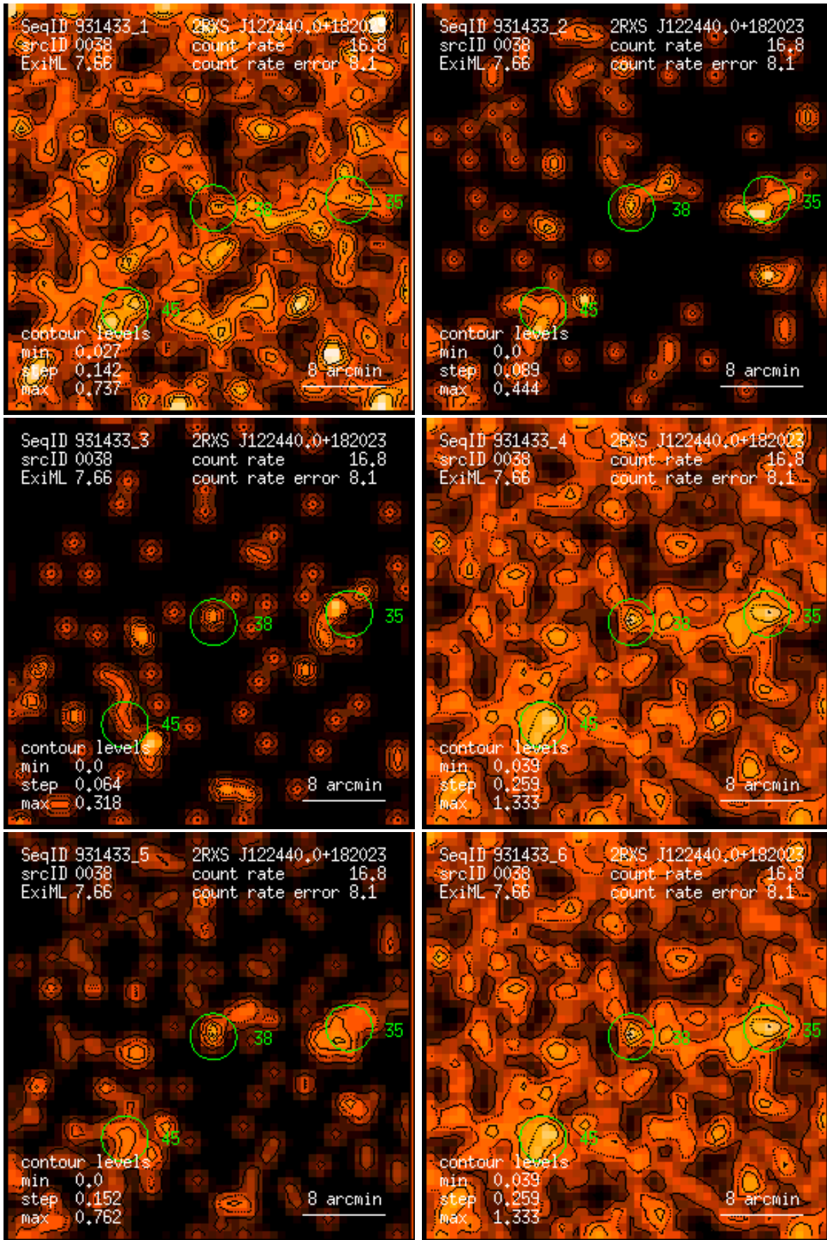
Figure 38: RASS 931433: detection 0038: band rate images, Gaussian filter: (1) PSPC channels 11 – 41, (2) 52 – 90, (3) 91 – 201, (4) 11 – 235, (5) 52 – 201, (6) 11 – 201. Broad band rates in counts/ks. Band rate contour levels in counts/ks/arcmin 2 .
