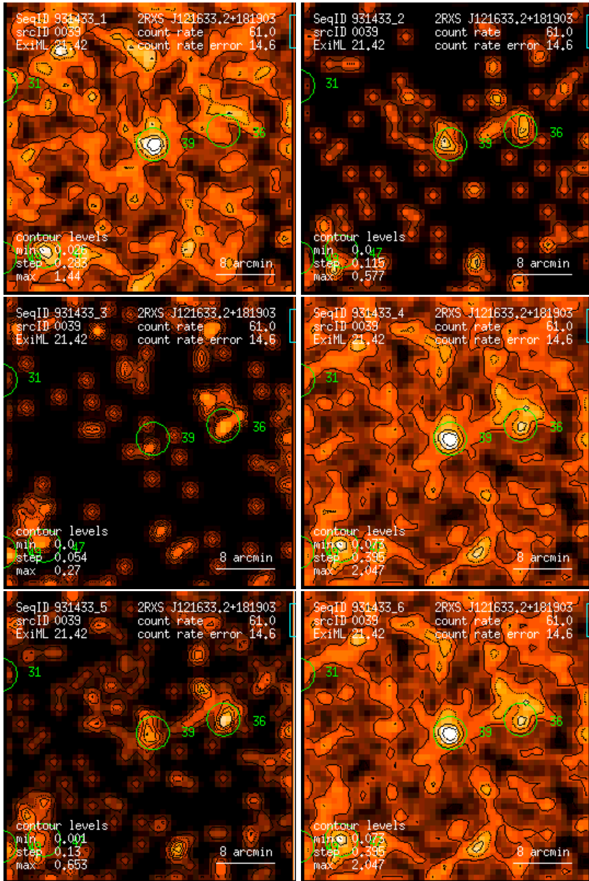
Figure 39: RASS 931433: detection 0039: band rate images, Gaussian filter: (1) PSPC channels 11 – 41, (2) 52 – 90, (3) 91 – 201, (4) 11 – 235, (5) 52 – 201, (6) 11 – 201. Broad band rates in counts/ks. Band rate contour levels in counts/ks/arcmin 2 .
