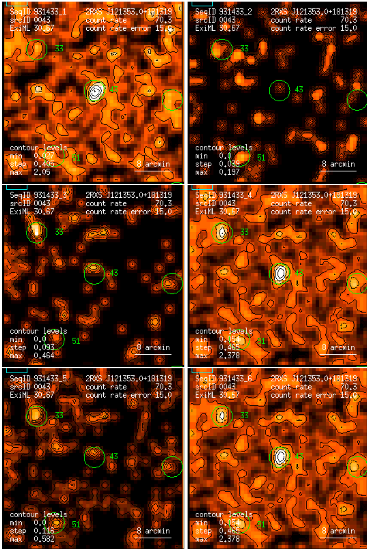
Figure 43: RASS 931433: detection 0043: band rate images, Gaussian filter: (1) PSPC channels 11 – 41, (2) 52 – 90, (3) 91 – 201, (4) 11 – 235, (5) 52 – 201, (6) 11 – 201. Broad band rates in counts/ks. Band rate contour levels in counts/ks/arcmin 2 .
