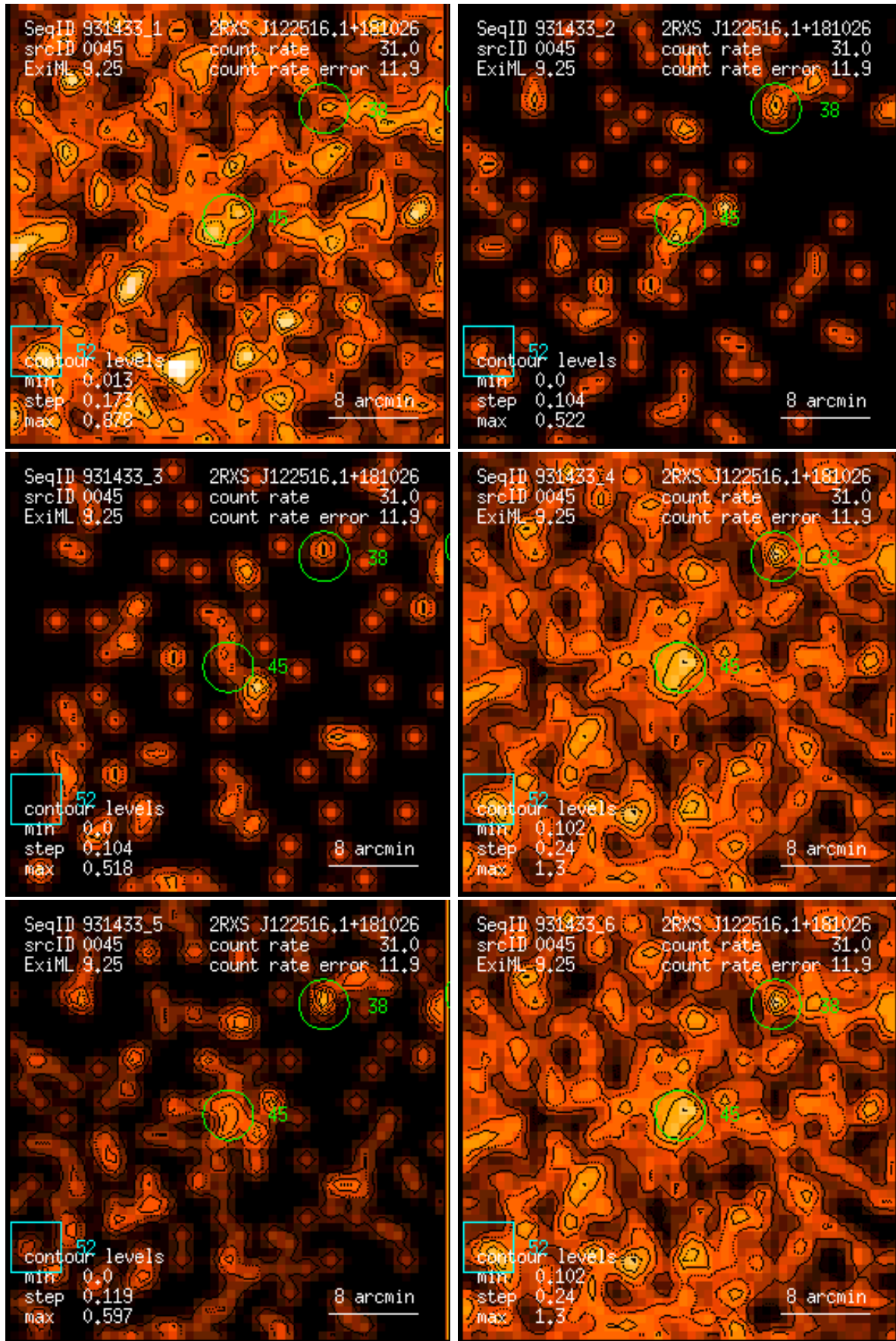
Figure 45: RASS 931433: detection 0045: band rate images, Gaussian filter: (1) PSPC channels 11 – 41, (2) 52 – 90, (3) 91 – 201, (4) 11 – 235, (5) 52 – 201, (6) 11 – 201. Broad band rates in counts/ks. Band rate contour levels in counts/ks/arcmin 2 .
