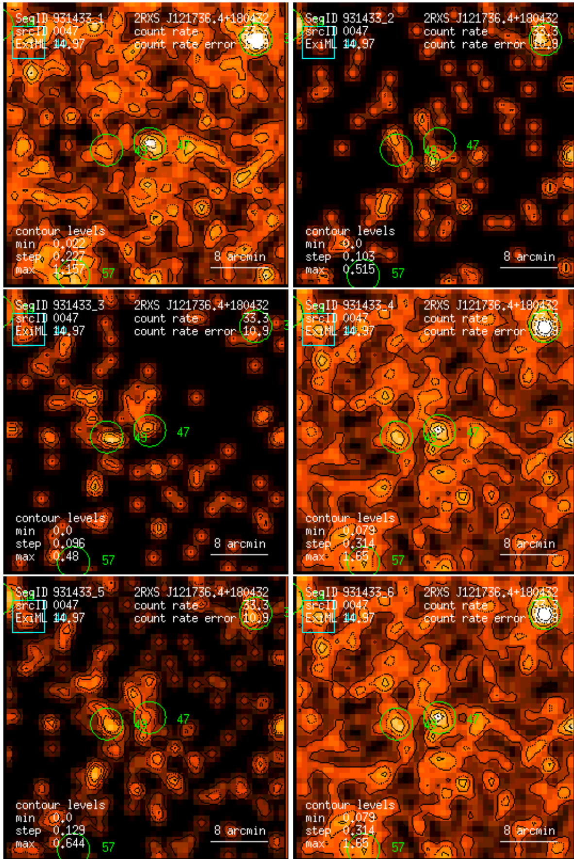
Figure 47: RASS 931433: detection 0047: band rate images, Gaussian filter: (1) PSPC channels 11 – 41, (2) 52 – 90, (3) 91 – 201, (4) 11 – 235, (5) 52 – 201, (6) 11 – 201. Broad band rates in counts/ks. Band rate contour levels in counts/ks/arcmin 2 .
