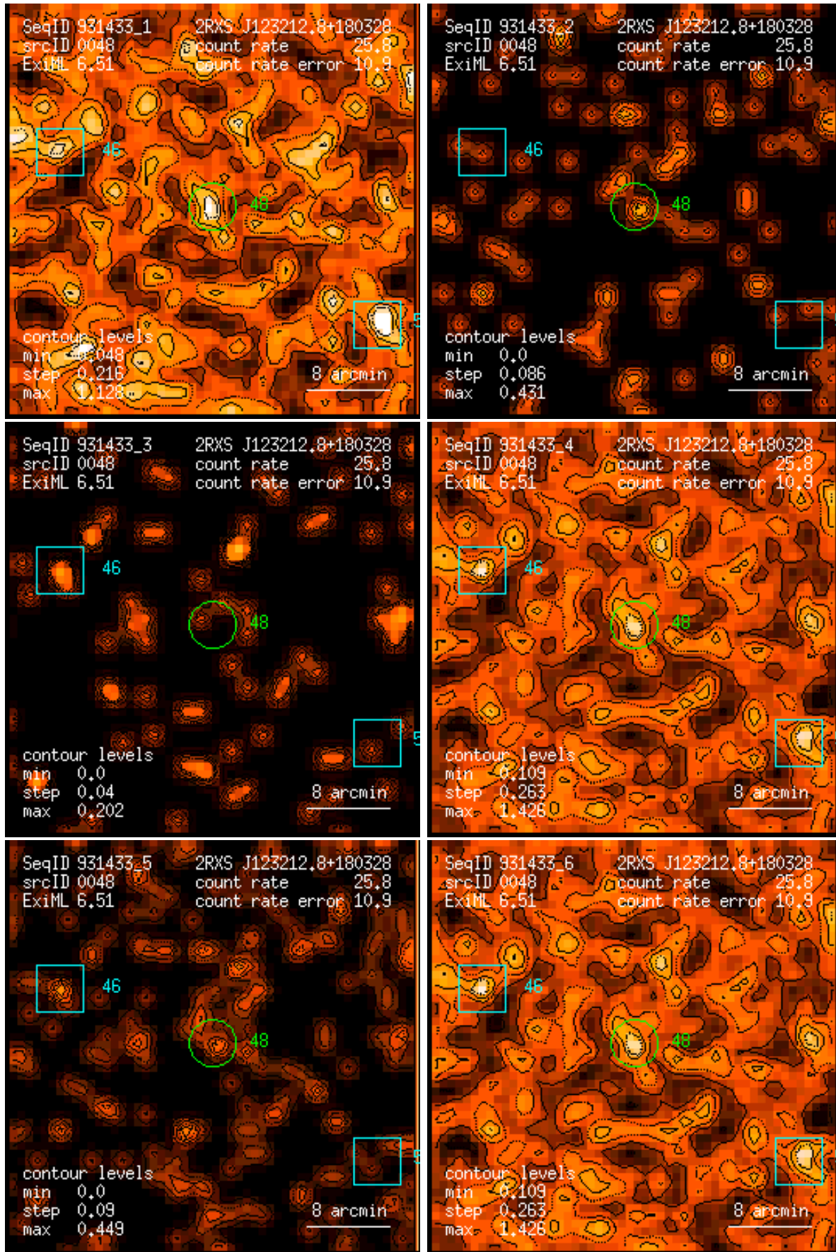
Figure 48: RASS 931433: detection 0048: band rate images, Gaussian filter: (1) PSPC channels 11 – 41, (2) 52 – 90, (3) 91 – 201, (4) 11 – 235, (5) 52 – 201, (6) 11 – 201. Broad band rates in counts/ks. Band rate contour levels in counts/ks/arcmin 2 .
