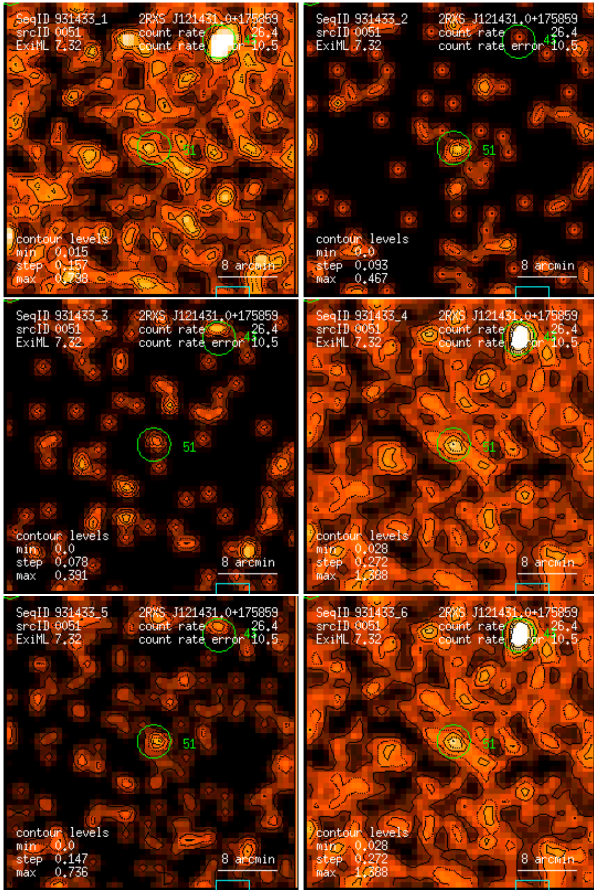
Figure 51: RASS 931433: detection 0051: band rate images, Gaussian filter: (1) PSPC channels 11 – 41, (2) 52 – 90, (3) 91 – 201, (4) 11 – 235, (5) 52 – 201, (6) 11 – 201. Broad band rates in counts/ks. Band rate contour levels in counts/ks/arcmin 2 .
