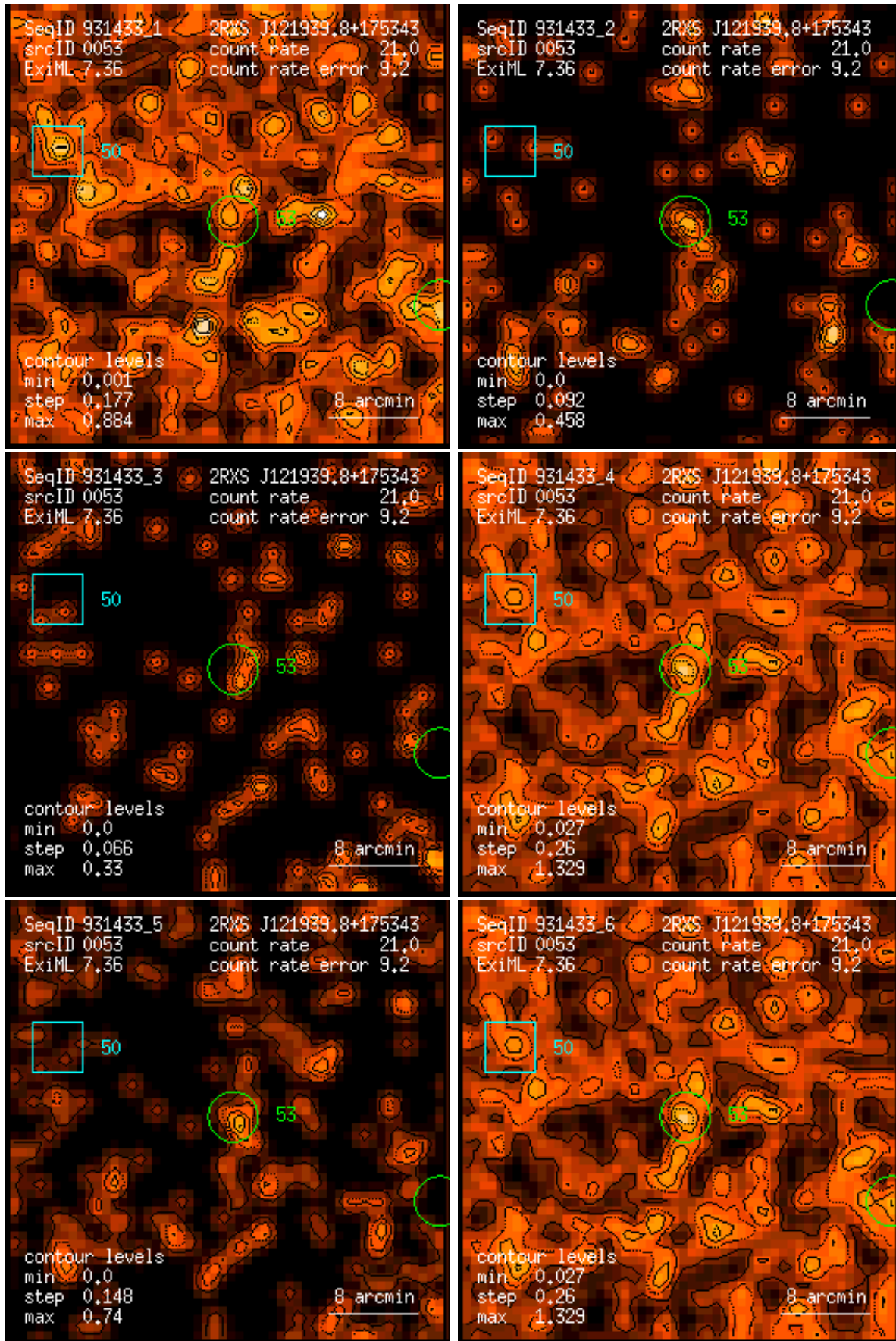
Figure 53: RASS 931433: detection 0053: band rate images, Gaussian filter: (1) PSPC channels 11 – 41, (2) 52 – 90, (3) 91 – 201, (4) 11 – 235, (5) 52 – 201, (6) 11 – 201. Broad band rates in counts/ks. Band rate contour levels in counts/ks/arcmin 2 .
