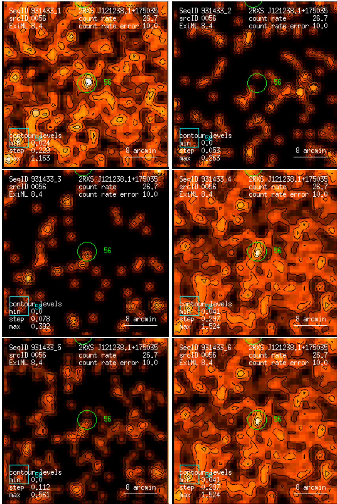
Figure 56: RASS 931433: detection 0056: band rate images, Gaussian filter: (1) PSPC channels 11 – 41, (2) 52 – 90, (3) 91 – 201, (4) 11 – 235, (5) 52 – 201, (6) 11 – 201. Broad band rates in counts/ks. Band rate contour levels in counts/ks/arcmin 2 .
