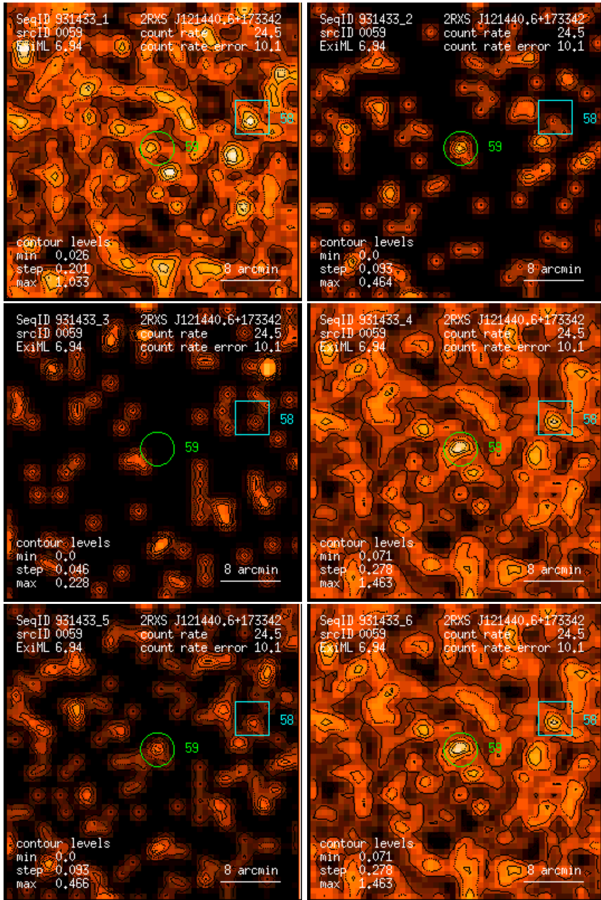
Figure 59: RASS 931433: detection 0059: band rate images, Gaussian filter: (1) PSPC channels 11 – 41, (2) 52 – 90, (3) 91 – 201, (4) 11 – 235, (5) 52 – 201, (6) 11 – 201. Broad band rates in counts/ks. Band rate contour levels in counts/ks/arcmin 2 .
