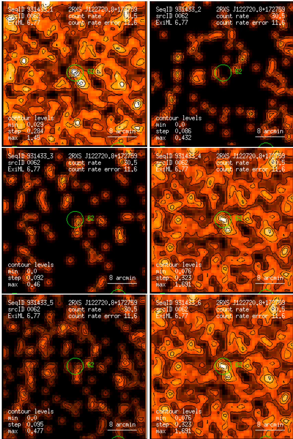
Figure 62: RASS 931433: detection 0062: band rate images, Gaussian filter: (1) PSPC channels 11 – 41, (2) 52 – 90, (3) 91 – 201, (4) 11 – 235, (5) 52 – 201, (6) 11 – 201. Broad band rates in counts/ks. Band rate contour levels in counts/ks/arcmin 2 .
