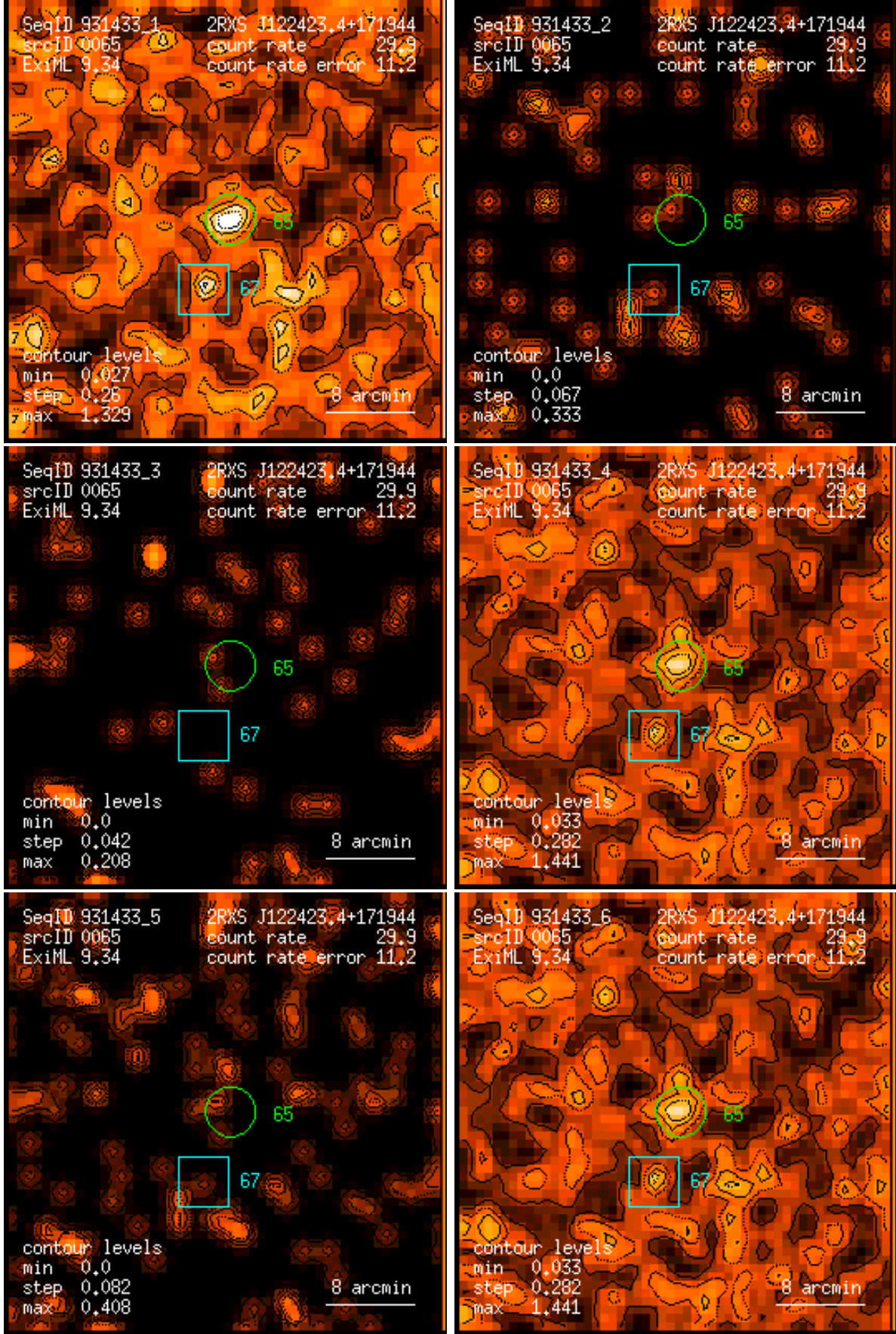
Figure 65: RASS 931433: detection 0065: band rate images, Gaussian filter: (1) PSPC channels 11 – 41, (2) 52 – 90, (3) 91 – 201, (4) 11 – 235, (5) 52 – 201, (6) 11 – 201. Broad band rates in counts/ks. Band rate contour levels in counts/ks/arcmin 2 .
