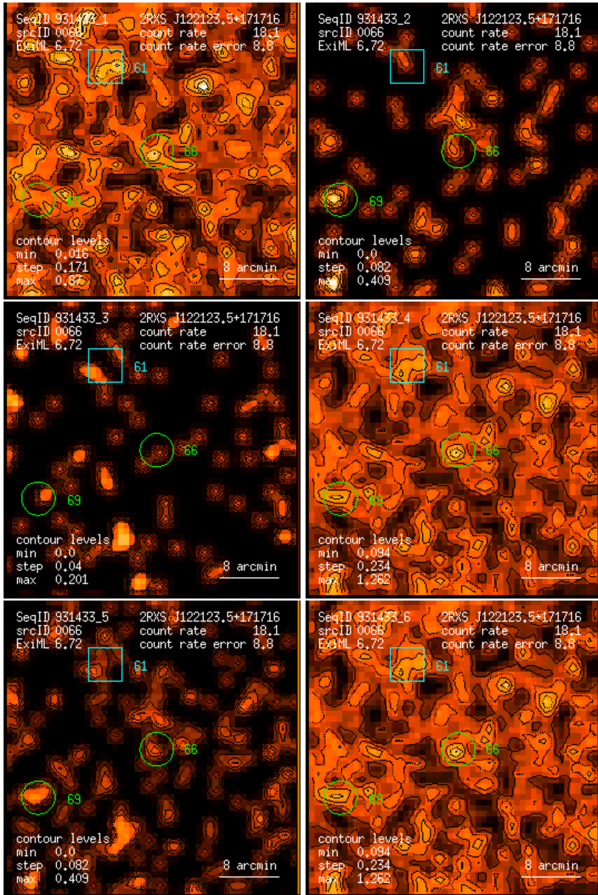
Figure 66: RASS 931433: detection 0066: band rate images, Gaussian filter: (1) PSPC channels 11 – 41, (2) 52 – 90, (3) 91 – 201, (4) 11 – 235, (5) 52 – 201, (6) 11 – 201. Broad band rates in counts/ks. Band rate contour levels in counts/ks/arcmin 2 .
