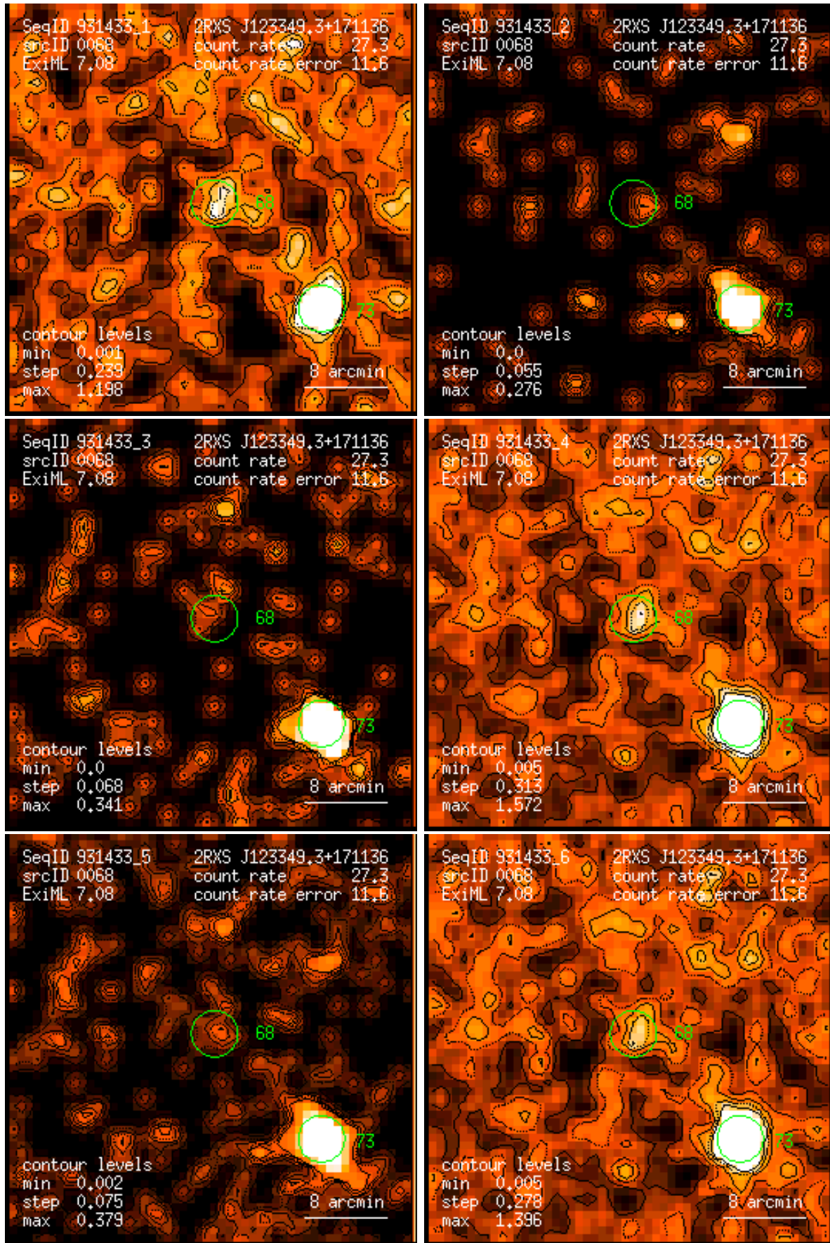
Figure 68: RASS 931433: detection 0068: band rate images, Gaussian filter: (1) PSPC channels 11 – 41, (2) 52 – 90, (3) 91 – 201, (4) 11 – 235, (5) 52 – 201, (6) 11 – 201. Broad band rates in counts/ks. Band rate contour levels in counts/ks/arcmin 2 .
