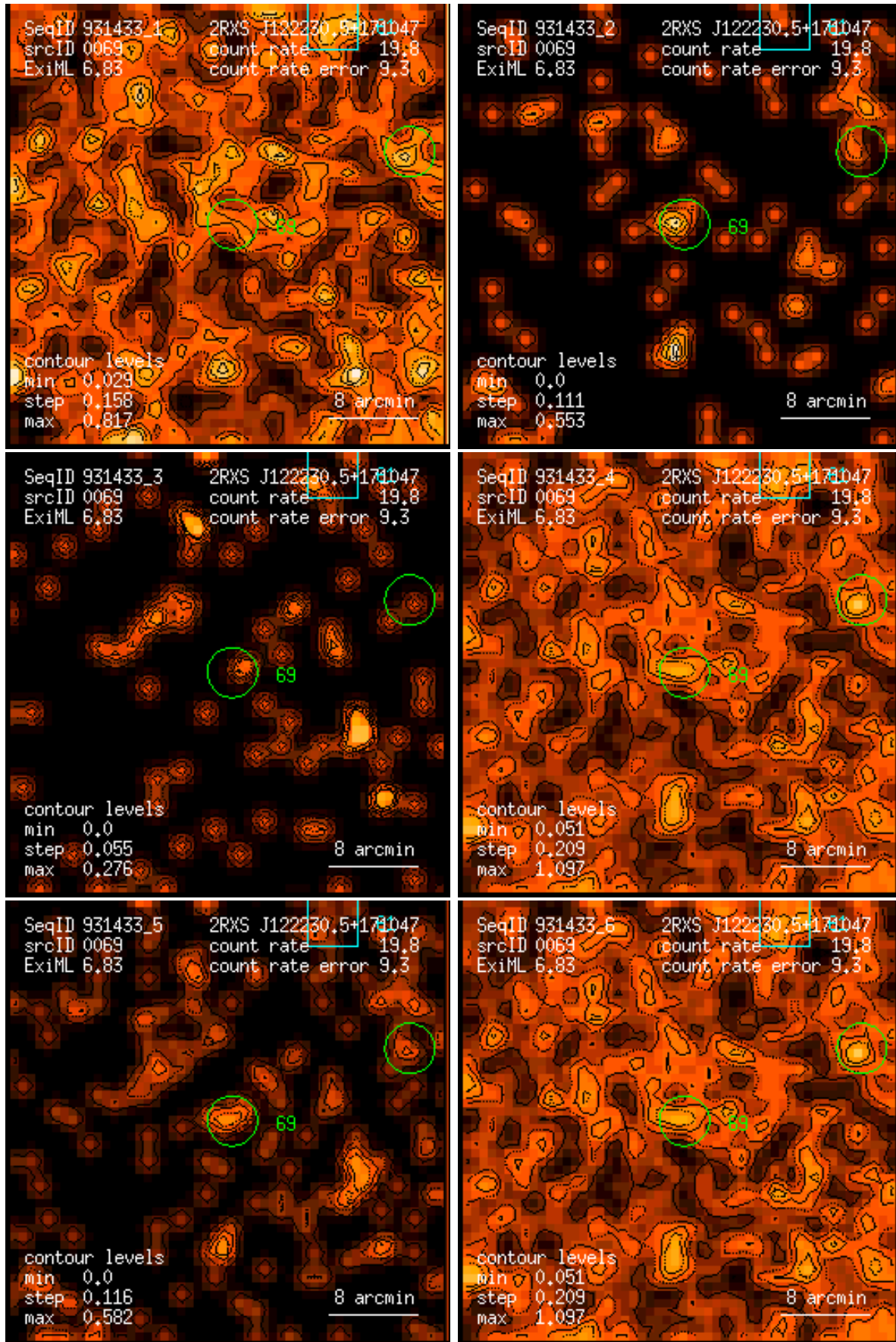
Figure 69: RASS 931433: detection 0069: band rate images, Gaussian filter: (1) PSPC channels 11 – 41, (2) 52 – 90, (3) 91 – 201, (4) 11 – 235, (5) 52 – 201, (6) 11 – 201. Broad band rates in counts/ks. Band rate contour levels in counts/ks/arcmin 2 .
