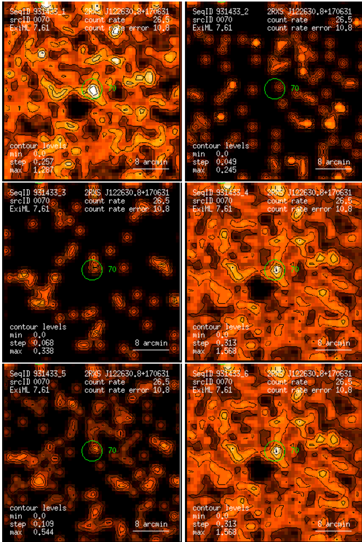
Figure 70: RASS 931433: detection 0070: band rate images, Gaussian filter: (1) PSPC channels 11 – 41, (2) 52 – 90, (3) 91 – 201, (4) 11 – 235, (5) 52 – 201, (6) 11 – 201. Broad band rates in counts/ks. Band rate contour levels in counts/ks/arcmin 2 .
