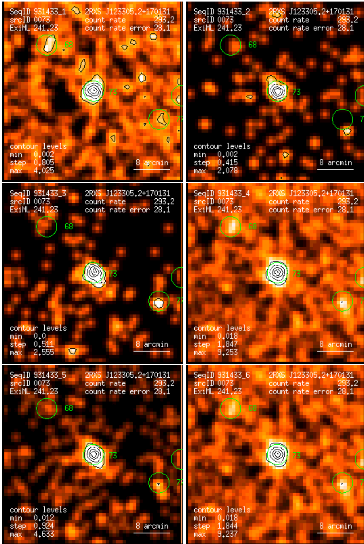
Figure 73: RASS 931433: detection 0073: band rate images, Gaussian filter: (1) PSPC channels 11 – 41, (2) 52 – 90, (3) 91 – 201, (4) 11 – 235, (5) 52 – 201, (6) 11 – 201. Broad band rates in counts/ks. Band rate contour levels in counts/ks/arcmin 2 .
