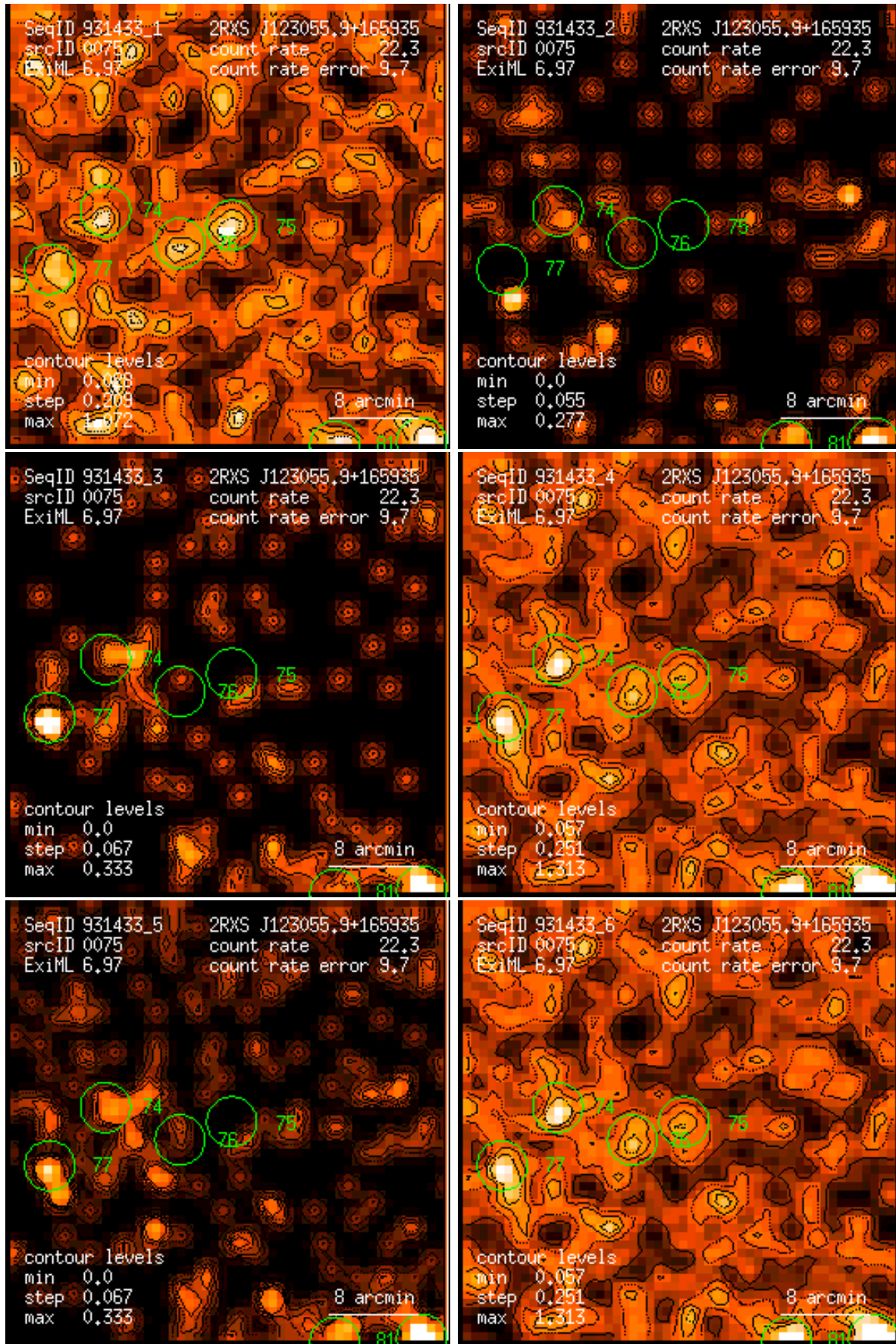
Figure 75: RASS 931433: detection 0075: band rate images, Gaussian filter: (1) PSPC channels 11 – 41, (2) 52 – 90, (3) 91 – 201, (4) 11 – 235, (5) 52 – 201, (6) 11 – 201. Broad band rates in counts/ks. Band rate contour levels in counts/ks/arcmin 2 .
