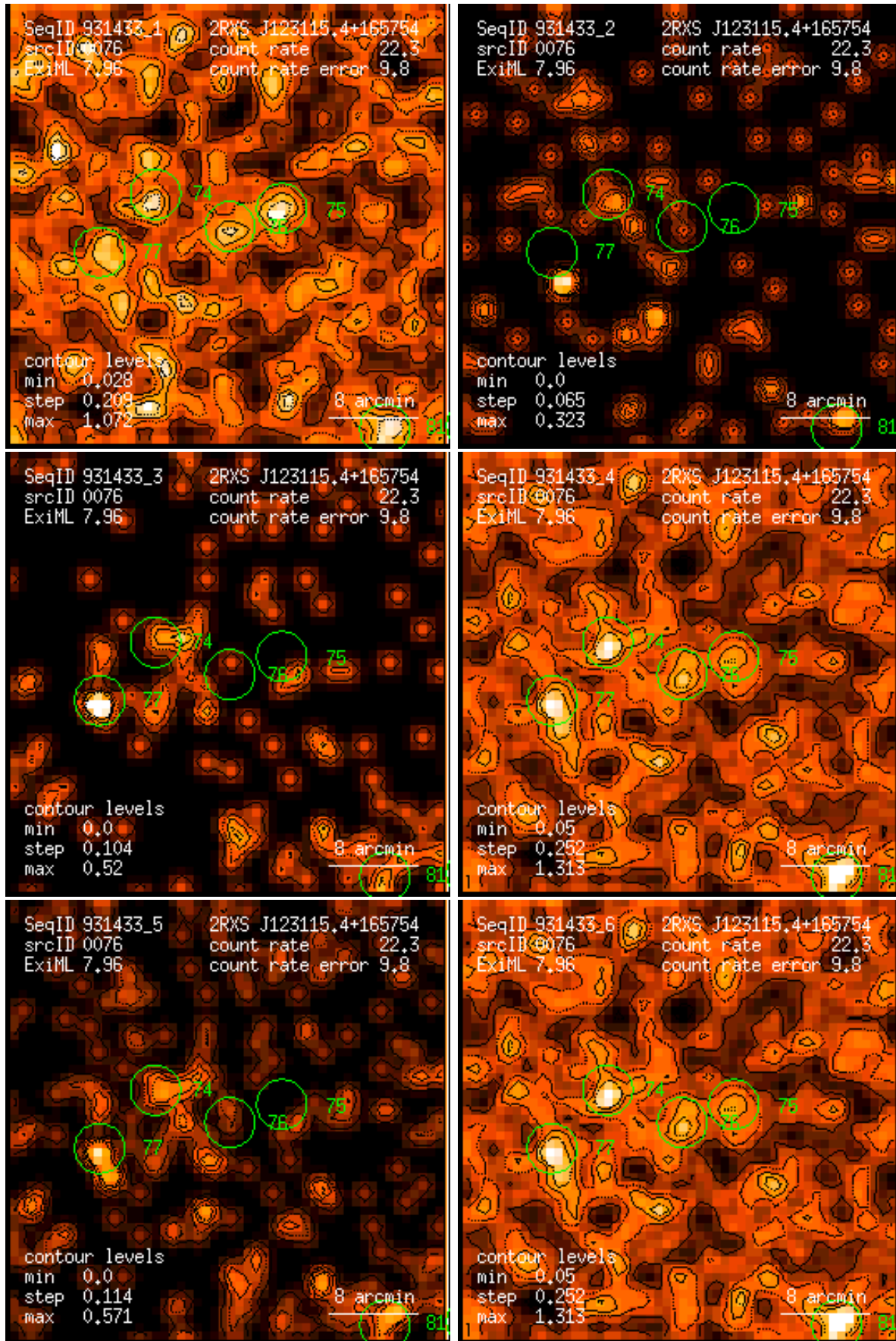
Figure 76: RASS 931433: detection 0076: band rate images, Gaussian filter: (1) PSPC channels 11 – 41, (2) 52 – 90, (3) 91 – 201, (4) 11 – 235, (5) 52 – 201, (6) 11 – 201. Broad band rates in counts/ks. Band rate contour levels in counts/ks/arcmin 2 .
