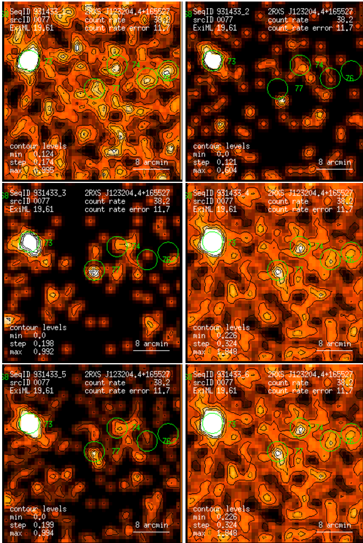
Figure 77: RASS 931433: detection 0077: band rate images, Gaussian filter: (1) PSPC channels 11 – 41, (2) 52 – 90, (3) 91 – 201, (4) 11 – 235, (5) 52 – 201, (6) 11 – 201. Broad band rates in counts/ks. Band rate contour levels in counts/ks/arcmin 2 .
