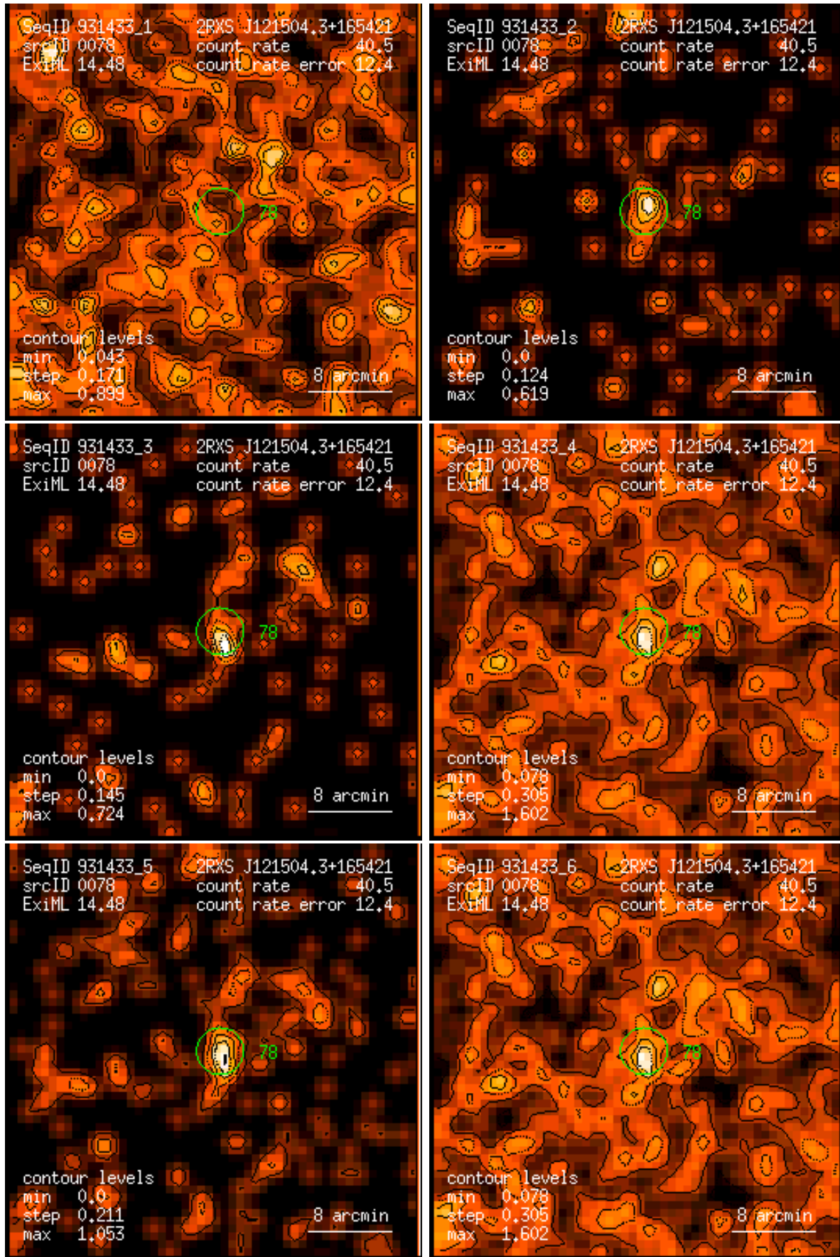
Figure 78: RASS 931433: detection 0078: band rate images, Gaussian filter: (1) PSPC channels 11 – 41, (2) 52 – 90, (3) 91 – 201, (4) 11 – 235, (5) 52 – 201, (6) 11 – 201. Broad band rates in counts/ks. Band rate contour levels in counts/ks/arcmin 2 .
