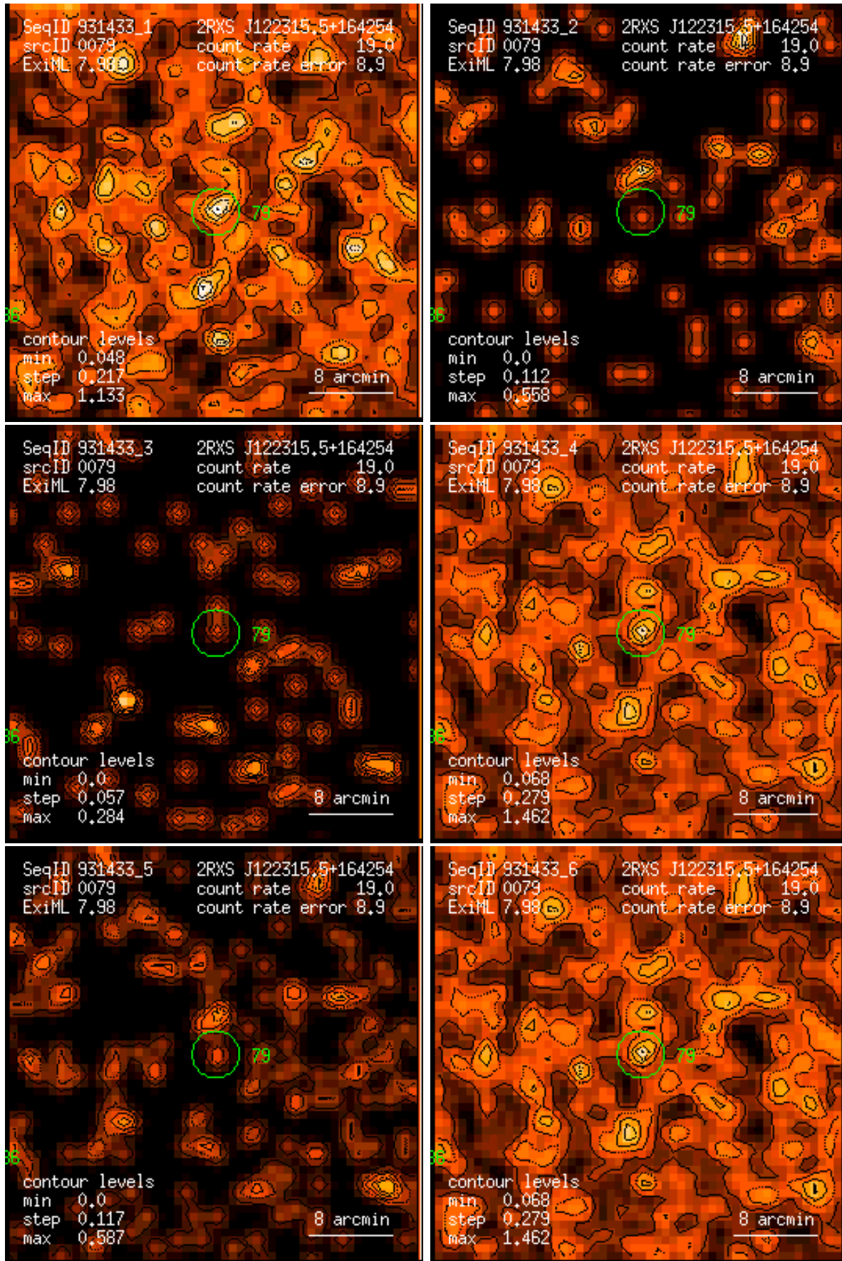
Figure 79: RASS 931433: detection 0079: band rate images, Gaussian filter: (1) PSPC channels 11 – 41, (2) 52 – 90, (3) 91 – 201, (4) 11 – 235, (5) 52 – 201, (6) 11 – 201. Broad band rates in counts/ks. Band rate contour levels in counts/ks/arcmin 2 .
