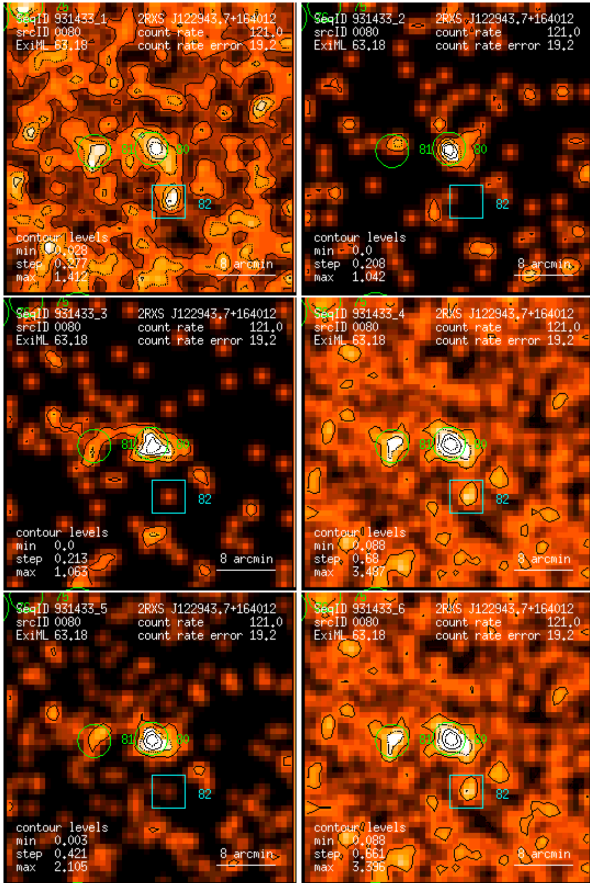
Figure 80: RASS 931433: detection 0080: band rate images, Gaussian filter: (1) PSPC channels 11 – 41, (2) 52 – 90, (3) 91 – 201, (4) 11 – 235, (5) 52 – 201, (6) 11 – 201. Broad band rates in counts/ks. Band rate contour levels in counts/ks/arcmin 2 .
