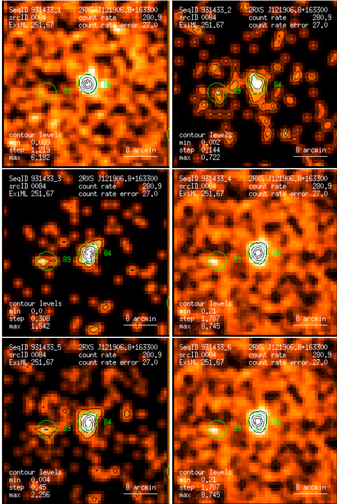
Figure 84: RASS 931433: detection 0084: band rate images, Gaussian filter: (1) PSPC channels 11 – 41, (2) 52 – 90, (3) 91 – 201, (4) 11 – 235, (5) 52 – 201, (6) 11 – 201. Broad band rates in counts/ks. Band rate contour levels in counts/ks/arcmin 2 .
