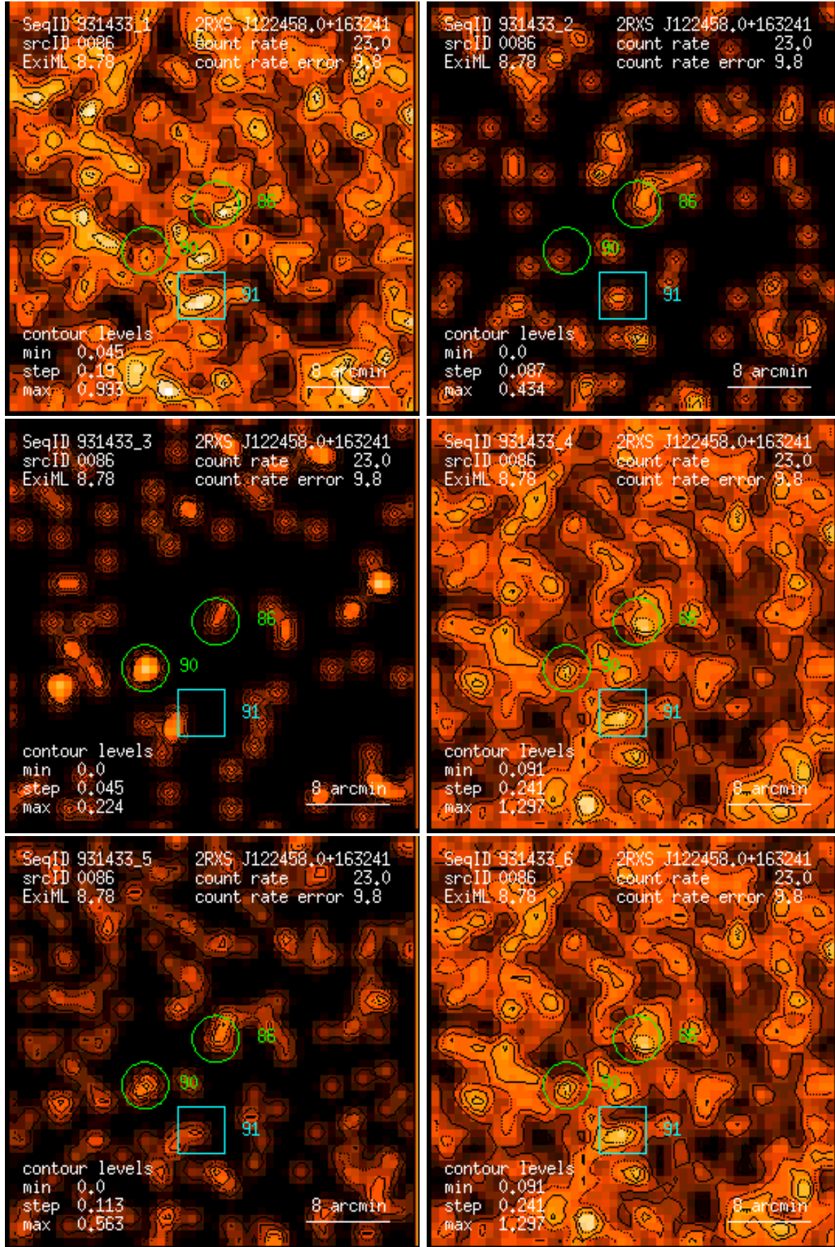
Figure 86: RASS 931433: detection 0086: band rate images, Gaussian filter: (1) PSPC channels 11 – 41, (2) 52 – 90, (3) 91 – 201, (4) 11 – 235, (5) 52 – 201, (6) 11 – 201. Broad band rates in counts/ks. Band rate contour levels in counts/ks/arcmin 2 .
