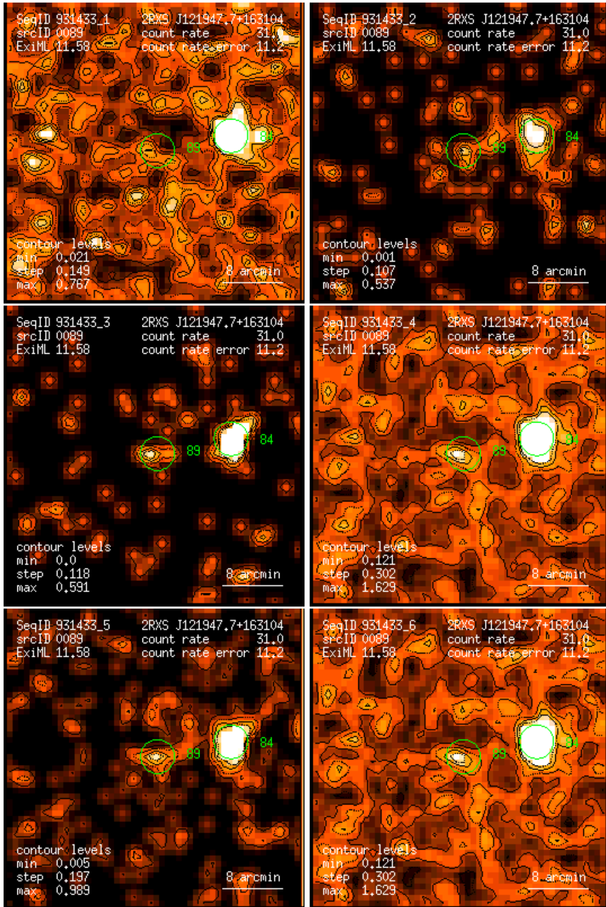
Figure 89: RASS 931433: detection 0089: band rate images, Gaussian filter: (1) PSPC channels 11 – 41, (2) 52 – 90, (3) 91 – 201, (4) 11 – 235, (5) 52 – 201, (6) 11 – 201. Broad band rates in counts/ks. Band rate contour levels in counts/ks/arcmin 2 .
