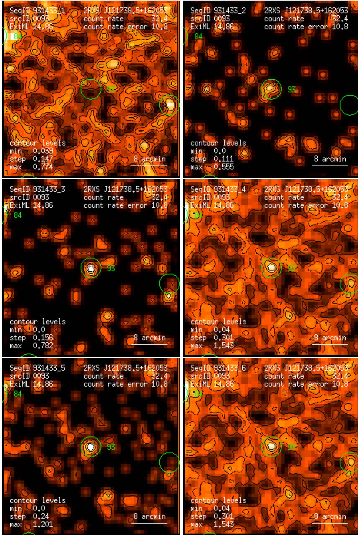
Figure 93: RASS 931433: detection 0093: band rate images, Gaussian filter: (1) PSPC channels 11 – 41, (2) 52 – 90, (3) 91 – 201, (4) 11 – 235, (5) 52 – 201, (6) 11 – 201. Broad band rates in counts/ks. Band rate contour levels in counts/ks/arcmin 2 .
